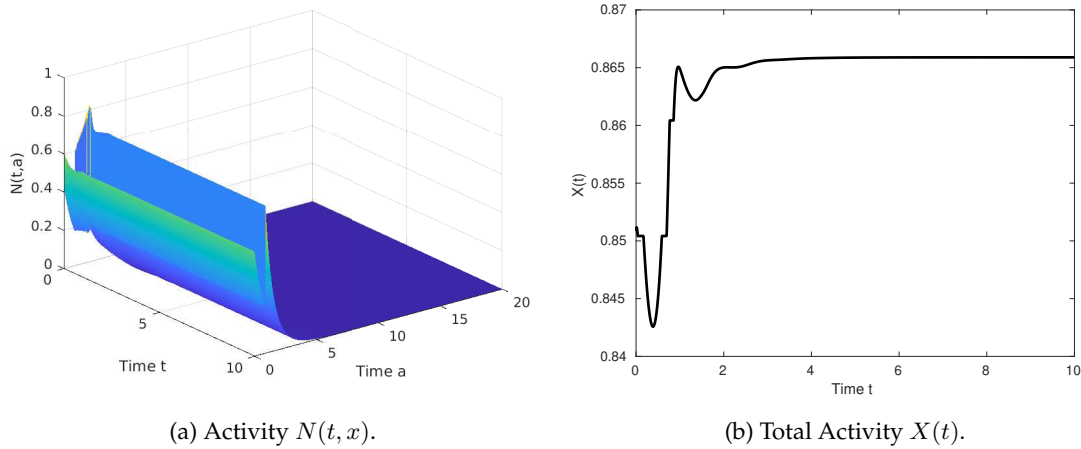
Figure 4: Example 1. Case n_0(s, a) = e^{-a} and p = \mathbb{1}_{\{s > X\}} + \mathbb{1}_{\{s-a > X\}} .
