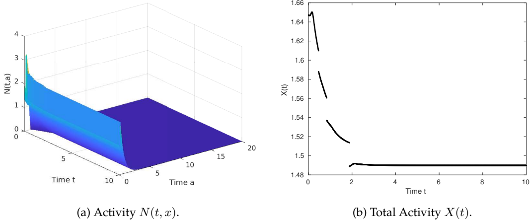
Figure 5: Example 2. Case n_0(s, a) = 2 \cdot \mathbb{1}_{\{2>a>s+1\}} and p = \mathbb{1}_{\{s>e^{-x}\}} + \mathbb{1}_{\{s-a>e^{-x}\}} .
