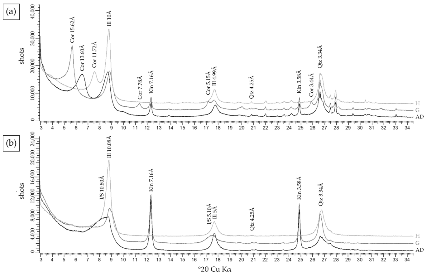
Figure 9. XRD patterns obtained for the clay fraction <2\mu\text{m} in Air-Dried (AD), Glycolated (G) and Heated (H) for the NH granite and showing the clay composition of the samples in the NH granite: (a) corrensite (Cor), a chlorite/smectite mixed-layer, and (b) illite/smectite mixed-layer (I/S). Abbreviations (except for “Cor and I/S”) after [45]: Bt—Biotite, Kln—Kaolinite, Qtz—Quartz, Ill—Illite.
