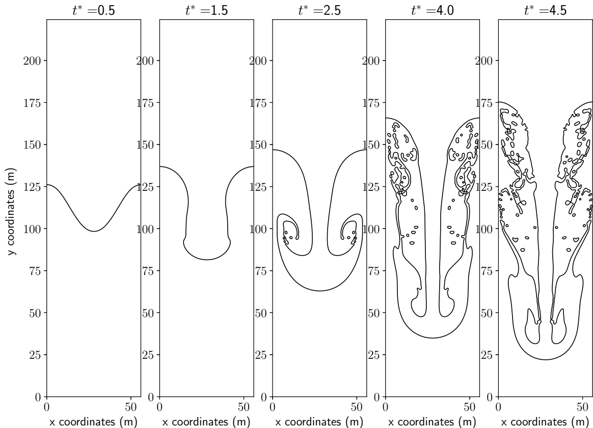
Figure 8: Rayleigh-Taylor instability at various characteristic times t^* , Reynolds number is Re = 2048
