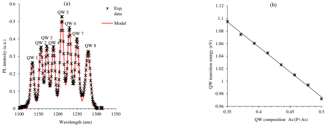
Figure 2. (a) PL spectrum measured at 10 K with 1064 nm excitation after epitaxial growth (sample structure shown in fig. 1). Black symbols ( \star ): experimental data; full line (red): best-fit with the model described in text. (b) PL line energy versus QW composition. The full line in (b) is a linear best-fit to the PL energies.
