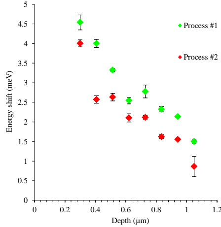
Figure 7. Energy shift of the QW transitions produced by the two etching processes.
