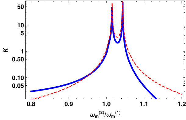
FIG. 10. Coefficient K of the contributions to J_{zx} that diverge like \omega_m^{(1)}/(\omega_c - \omega_{10}^{(2)}) [divided by the two coupling constants and the driving intensity g_{ec}^{(1)} g_{ec}^{(2)} A ] as a function of \omega_m^{(2)} . The solid line is the numerical result, and the dashed line is the analytical one, Eq. (43). The other parameters are g^{(1)} = g^{(2)} = 1.264\hbar\omega_m^{(1)} , t^{(1)} = 10\hbar\omega_m^{(1)} , and t^{(2)} = 10.5\hbar\omega_m^{(1)} .
