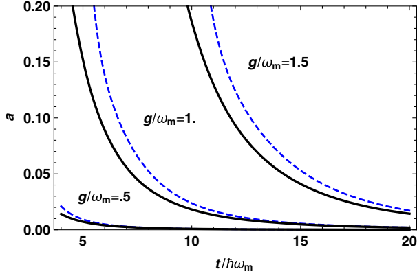
FIG. 6. Comparison between numerical (solid line) and analytical (dashed line) dependence of the anharmonicity parameter a for three values of the coupling g/\omega_m = 0.5, 1 , and 1.5 .
