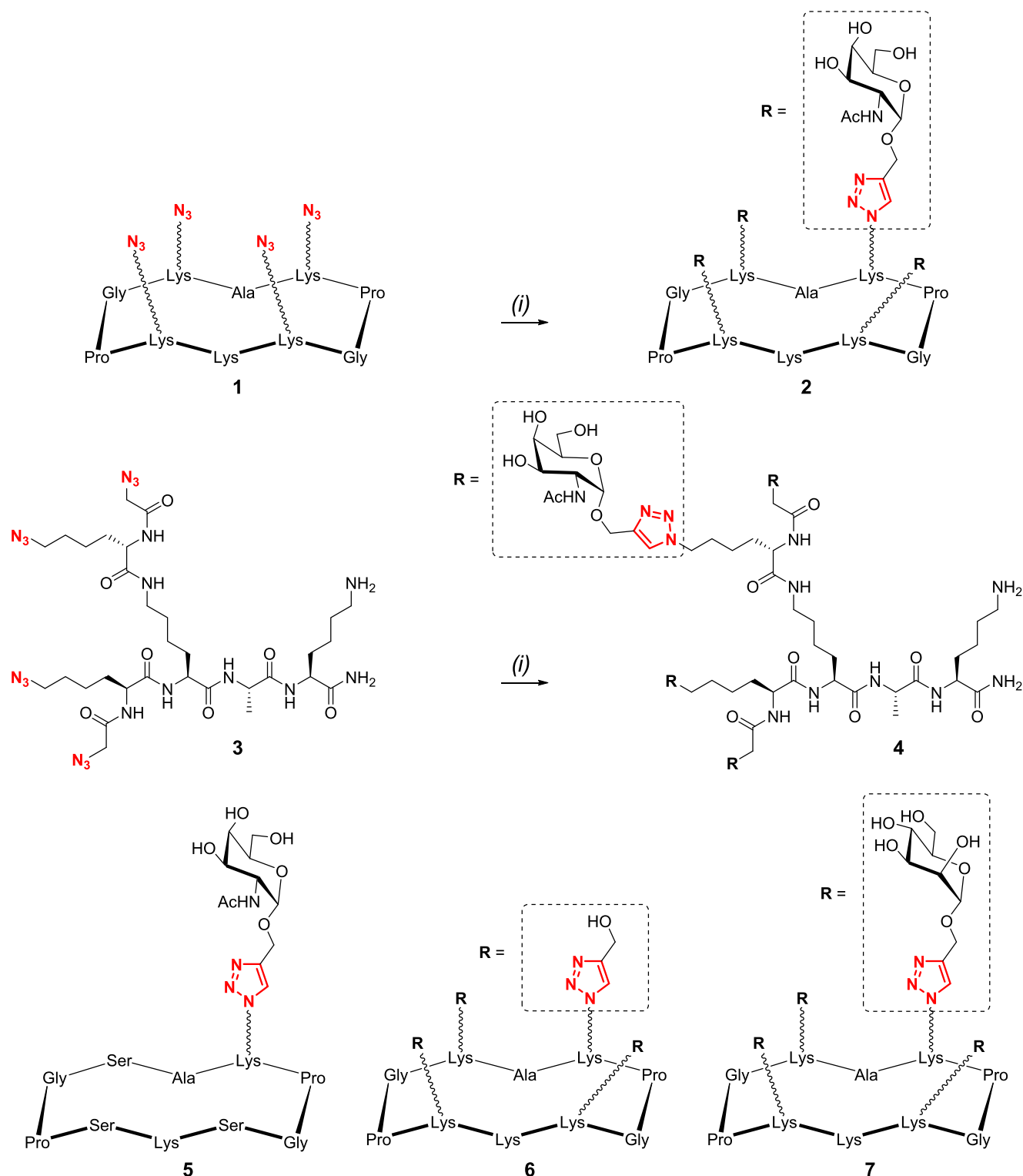
Scheme 1. Synthesis of Tetravalent Glycoclusters a
