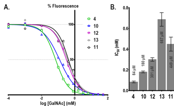
Figure 3. \text{IC}_{50} determination by competition with GalNAc incubated with HPA at 7.5 nM (immobilization concentration: 10 \mu\text{M} ): (A) inhibition curves; (B) \text{IC}_{50} values determined for the competitor.
