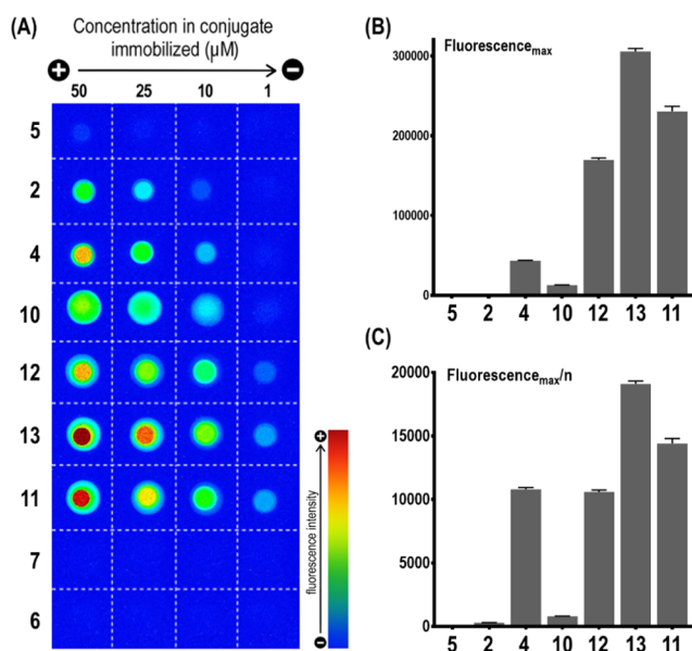
Figure 1. Fluorescence intensity evaluation for the interaction of multivalent glycoconjugates with HPA: (A) rainbow picture displaying fluorescence intensity (HPA: 1.9 nM, \lambda_{\text{ex}} = 635 nm); (B) comparison of the maximum of fluorescence (HPA: 7.5 nM; immobilization concentration of ligand: 40 \mu\text{M} ); and (C) comparison of the maximum of fluorescence normalized per monosaccharide unit (HPA: 7.5 nM; immobilization concentration of ligand: 40 \mu\text{M} ).
