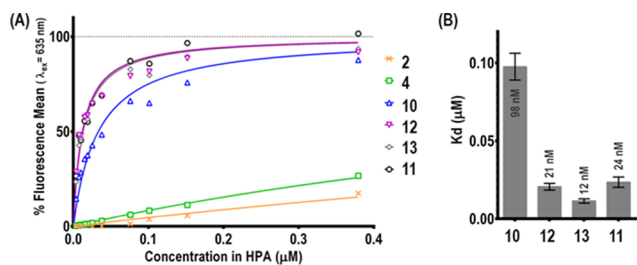
Figure 2. Determination of dissociation constants: (A) binding curves for the tetra- and hexadecavalent glycoconjugates (immobilization concentration: 10 \mu\text{M} ); (B) comparison of the dissociation constants for the hexadecavalent structures (mean of the K_d determined for a range of immobilization concentration of 40–0.3 \mu\text{M} ; see the Supporting Information).
