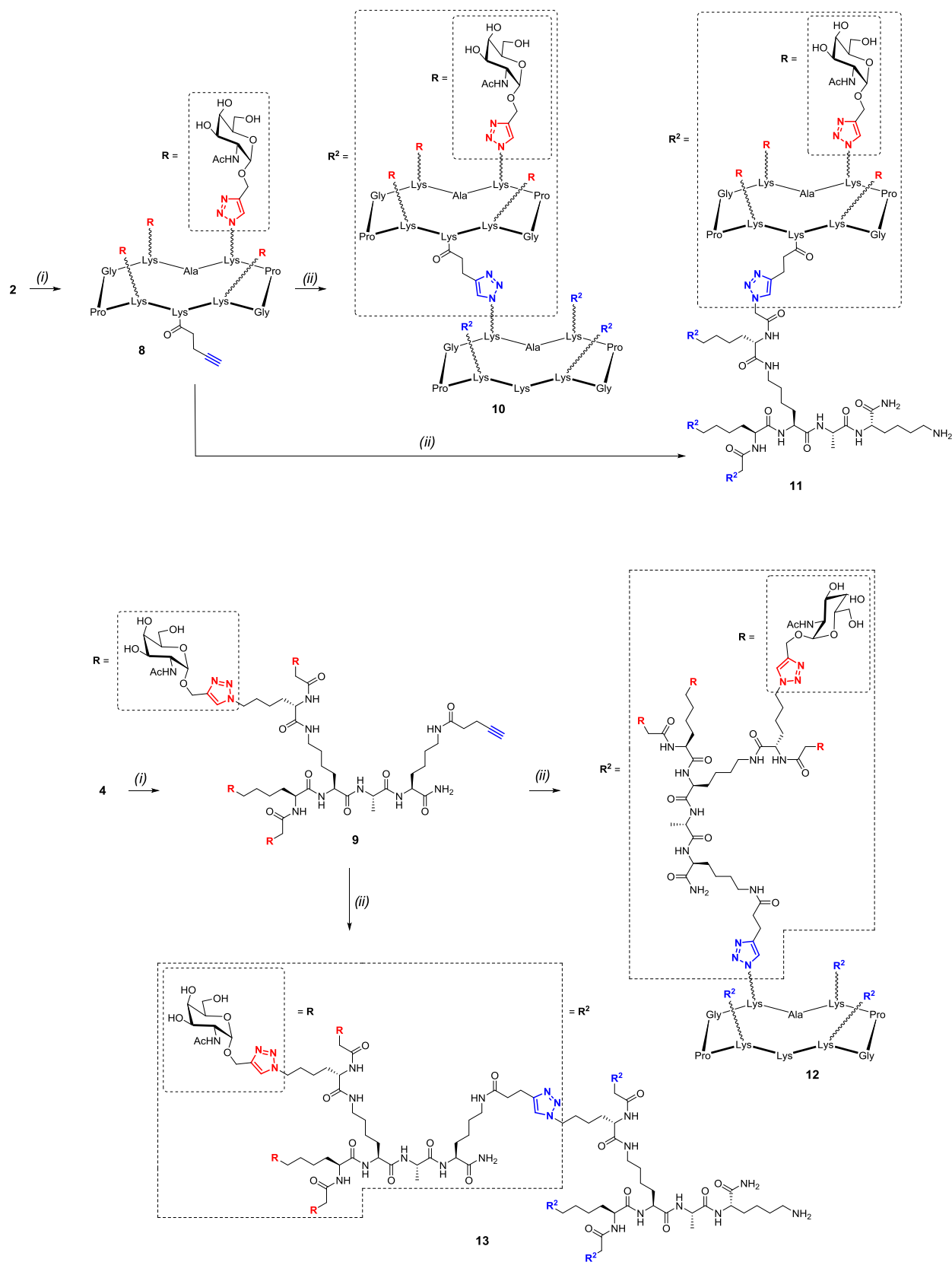
Scheme 2. Synthesis of Hexadecavalent Glycodendrimers a
