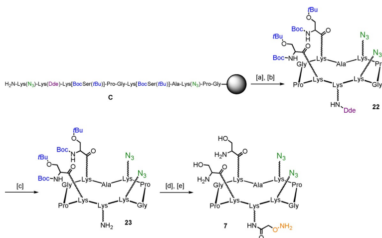
Scheme 4. Synthesis of "arm" cyclopeptide 7 . Reagents and conditions: [a] 1% TFA/ CH 2 Cl 2 , 10 × 10 min; [b] PyBOP ® (1.2 equiv), DIPEA (2.0 equiv), DMF/CH 2 Cl 2 (1:1), 0.5 mM linear peptide, r.t., 30 min, 55% overall; [c] 2% N 2 H 4 /DMF, r.t., 20 min., 94%; [d] (Boc-aminoxy)acetic acid N -hydroxysuccinimide ester (1.2 equiv), DIPEA (1.5 equiv), dry DMF, r.t., 20 min; [e] 94% TFA, 2% TIS, 2% H 2 O, 2% NH 2 OH, r.t., 3 h, 86% over two steps.
