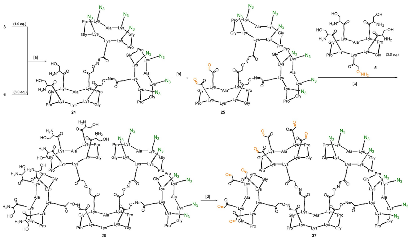
Scheme 5. Synthesis of multivalent scaffold 27 . Reagents and conditions: [a] 0.1% TFA in \text{H}_2\text{O}/\text{CH}_3\text{CN} (1:1), 37^\circ\text{C} , 30 min, 75%; [b] \text{NaIO}_4 (20 equiv), \text{H}_2\text{O} , r.t., 40 min, 70%; [c] 0.1% TFA in \text{H}_2\text{O}/\text{CH}_3\text{CN} (1:1), 37^\circ\text{C} , 30 min, 85%; [d] \text{NaIO}_4 (80 equiv), \text{H}_2\text{O} , r.t., 40 min, 78%.
