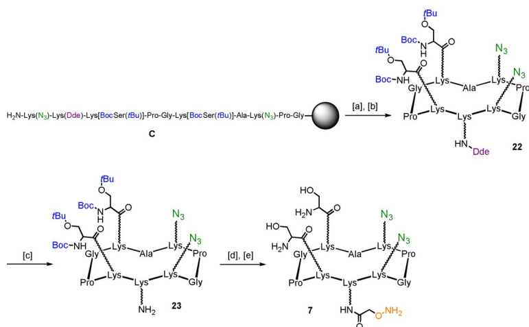
Scheme 4. Synthesis of "arm" cyclopeptide 7 . Reagents and conditions: [a] 1% TFA/ \text{CH}_2\text{Cl}_2 , 10 \times 10 min; [b] PyBOP ® (1.2 equiv), DIPEA (2.0 equiv), DMF/ \text{CH}_2\text{Cl}_2 (1:1), 0.5 mM linear peptide, r.t., 30 min, 55% overall; [c] 2% \text{N}_2\text{H}_4 /DMF, r.t., 20 min., 94%; [d] (Boc-aminoxy)acetic acid N -hydroxysuccinimide ester (1.2 equiv), DIPEA (1.5 equiv), dry DMF, r.t., 20 min; [e] 94% TFA, 2% TIS, 2% \text{H}_2\text{O} , 2% \text{NH}_2\text{OH} , r.t., 3 h, 86% over two steps.
