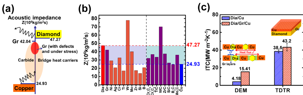
Fig. 8. (a) Acoustic impedance difference between diamond and Cu; (b) Comparison on reported acoustic impedance of metal coating and carbide [72]; (c) Results of ITC obtained from DEM calculations of the bulk Dia/Gr/Cu composite and from TDTR measurement of Dia/Gr/Cu model specimens.
