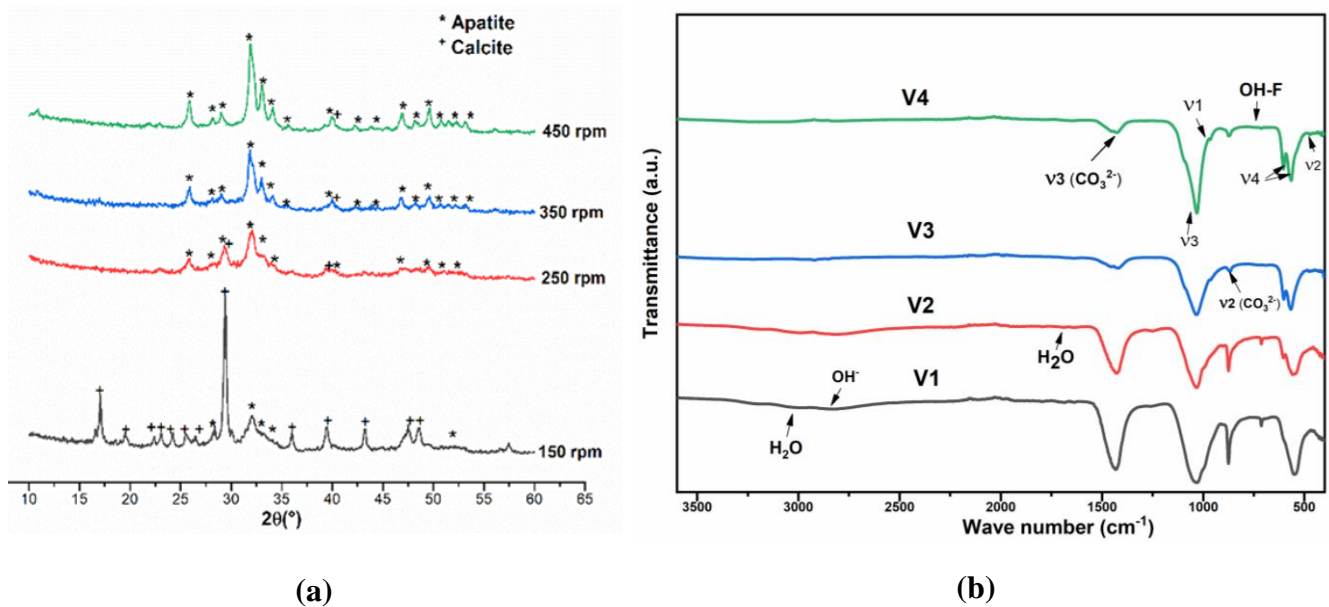
Fig. 2 (a) XRD patterns of synthesized samples as a function of the disc rotation speed (mp = 1.2g, 6 balls and 24 h); (b) IR spectra of samples prepared at different disc rotation speed (a. u. arbitrary units)
