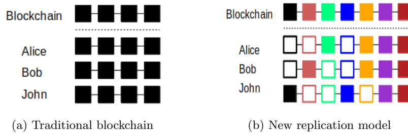
Fig. 2: Traditional blockchain vs the new replication model. In 2(a), each node maintains its chain which contains all previous transactions. Each given block is stored on the three nodes, Alice, Bob, and john. While in 2(b), the global blockchain shown at the top is sharded across the three nodes. Colored blocks represent the entire block containing transactions, and framed blocks only have the block header - so the block buried in the chain is held on a few nodes.
