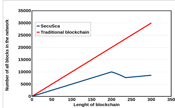
Fig. 5: Comparison of the size of blockchain between traditional blockchain and SecuSca
