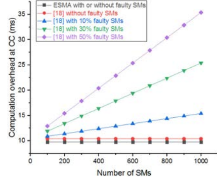
Fig. 6. FT decryption cost at CC.
