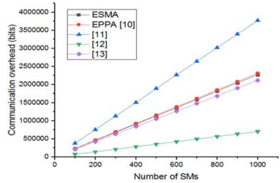
Fig. 7. SM-to-FN communication cost.
