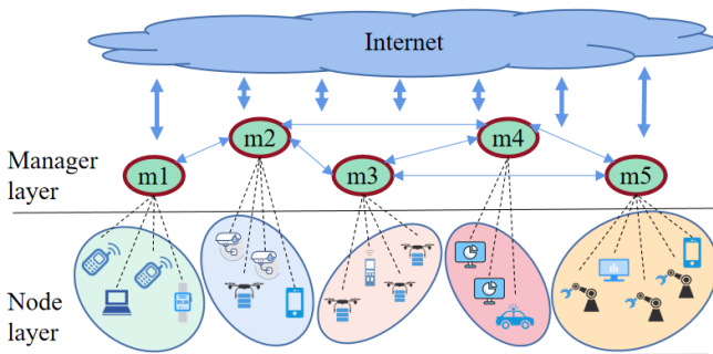
Fig. 1: Architecture of PDTM model
