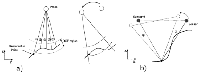
Figure 15: Modification of a scan direction due to: (a) DOF constraint, (b) occlusion problem [49].
