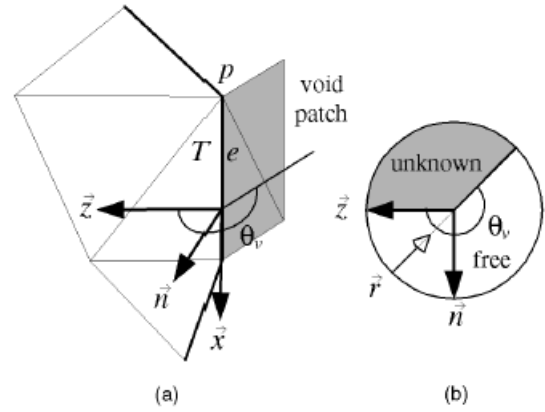
Figure 24: Efficient representation of the scanned and non-scanned areas: a) coordinate system of an edge, b) free space map induced by the scan orientation r [36].
