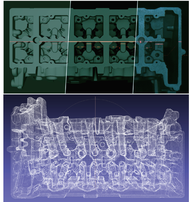
Figure 12: Top: (left) fast rasterization based simulation to evaluate the measurement coverage; (middle) simulations with path tracing, considering the camera spectral response; (right) real camera image. Bottom: Point cloud scanned by applying 30 acquisitions optimized through the greedy planning realized using the method of Mohammadikaji et al. [31].
