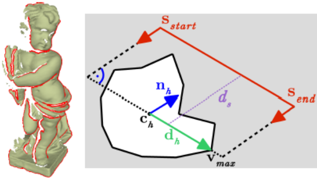
Figure 26: Viewpoint sampling method: left) boundaries detected in partial meshes of the Putto statue; right) a scan path in the direction of the largest expansion of the hole d_h , in the inverse hole normal n_h direction and at the optimal sensor distance d_s [21].
