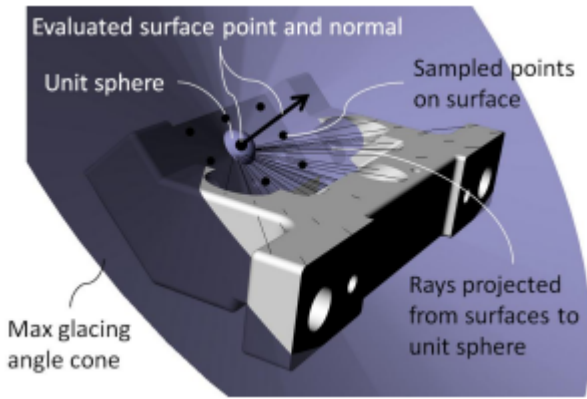
Figure 17: Determination of the visibility map. For a generic point, the occlusion produced by another surface was evaluated in the cone corresponding to the maximum glancing angle [39].
