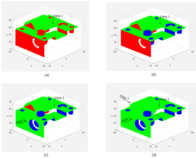
Figure 19: Result of an operation sequence generation: a) laser ability evaluation at the first iteration, b) after one iteration, c) after two iterations, and d) after three iterations. The green and blue regions indicate the surfaces measured using the laser sensor and touch probe, respectively, and the red region indicates the non-measured surface [40]
