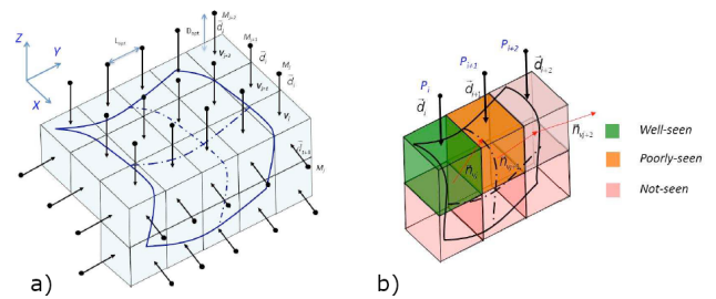
Figure 16: Representation of the initial set of viewpoints (a), and voxel qualification (b) [23].
