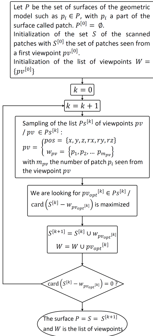
Figure 23: Formalization of the resolution steps for search based approaches
