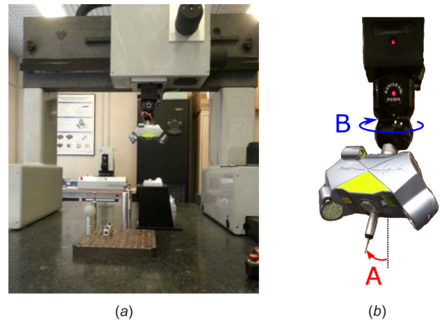
Figure 22: Configuration involving a CMM and hybrid sensor : a) view of the CMM, b) scanner KA50 composed of a touch probe and laser sensor mounted on a Renishaw PH10 head.
