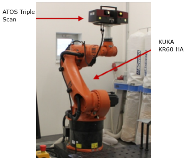
Figure 21: Configuration involving a KUKA robot arm and an ATOS structured light sensor [18].
