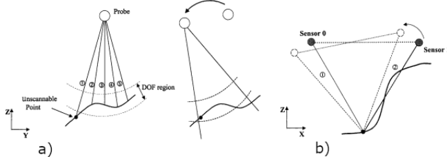
Figure 15: Modification of a scan direction due to: (a) DOF constraint, (b) occlusion problem [49].
