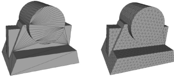
Figure 10: Original mesh (left) and mesh subdivided using the bubble mesh algorithm [47, 14] (right).
