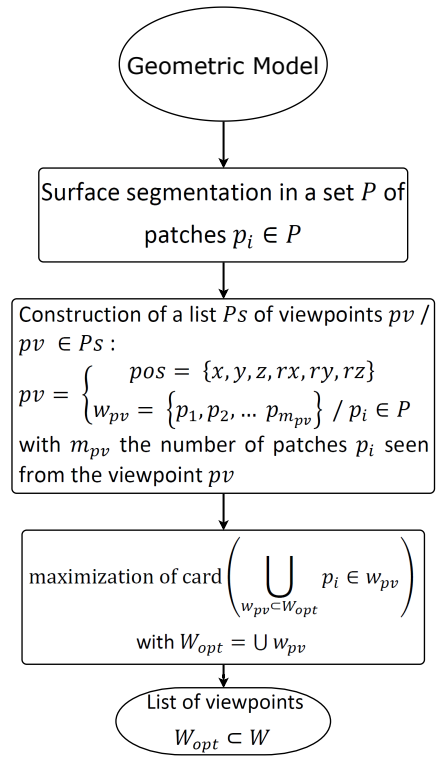
Figure 13: Formalization of the resolution steps for methods based on coverage optimization.
