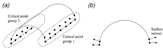
Figure 14: Critical point groups: (a) cylindrical surface, (b) cross-sectional view [25].
