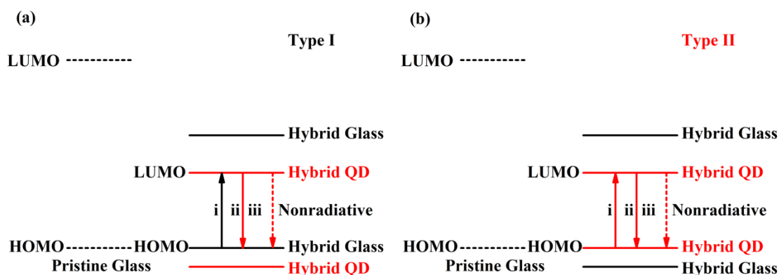
Figure 5 Energy diagrams demonstrating two different luminescence mechanism of CdSe quantum dot-doped glasses. The HOMO is determined by the hybrid glass in Type I (panel a) while it is decided by the hybrid QD in Type II (panel b).
