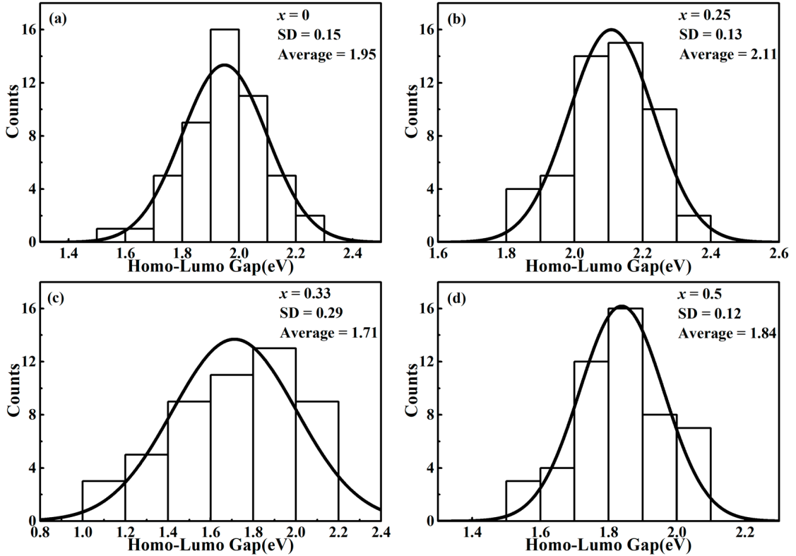
Figure 3 Histograms of HOMO–LUMO gap for CdSe quantum dot-doped sodium silicate glasses. The composition of the x Na 2 O–(1– x ) SiO 2 glass matrices: (a) x = 0 ; (b) x = 0.25 ; (c) x = 0.33 ; (d) x = 0.5 . A Gaussian function was used to fit the data and SD represent the standard deviation.
