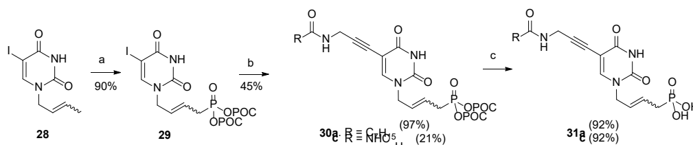
Scheme 4: reagents and conditions: (a) 25 , G-II, DCM Anh , 55 °C, 24 h.; (b) Pd(PPh 3 ) 4 , CuI, Et 3 N, alkynyl chains, DMF, rt, 16 h.; (c) NaOH (0.1 N), rt, 4 h, DOWEX 50WX8 (H + ).
