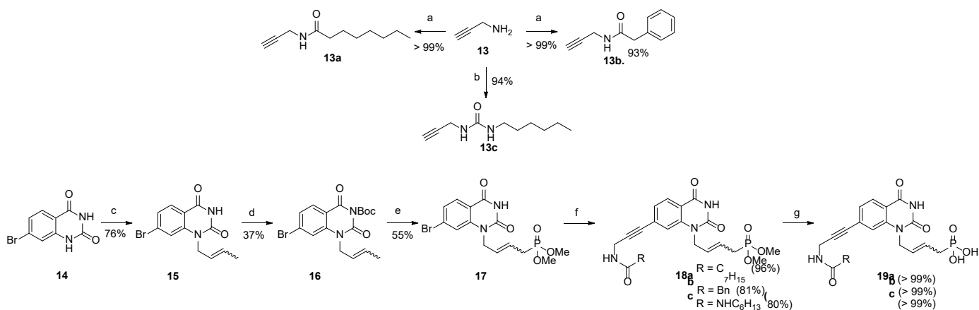
Scheme 2: reagents and conditions: (a) RCOCI, DIPEA, DCM anh , 0 °C-rt, 2 h.; (b) isocyanate DCM anh , 0 °C-rt, 2 h.; (c) (i) BSA, CH 3 CN, MW, 5 min, 80 °C, (ii) TMSCl, crotyl bromide, NaI act , MW, 30 min, 80 °C; (d) Boc 2 O, DMAP, THF, MW 70 °C, 10 min.; (e) (i) dimethyl-allylphosphonate, G-II, DCM anh , 80 KHz, 55 °C, 24 h, (ii) TFA, DCM, rt, 6 h.; (f) Pd(PPh 3 ) 4 , CuI, Et 3 N, alkynes 13a , 13b and 13c , DMF, 70 °C, 3 h.; (g) TMSBr, ACN anh , rt, 6 h.
