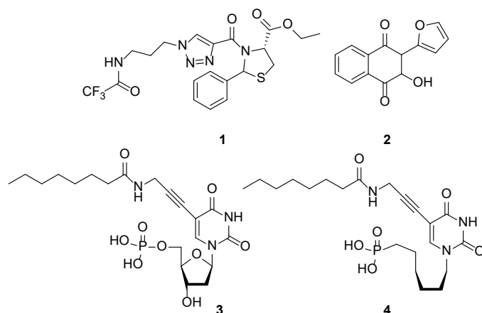
Fig. 1. Structures of FDTS inhibitors
