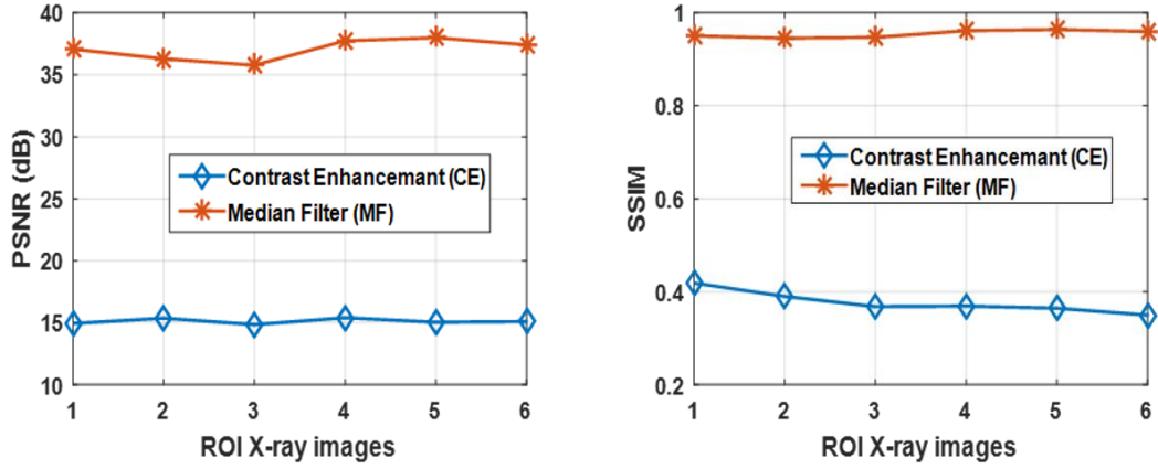
Fig. 7 Performance evaluation of contrast enhancement (CE) versus median filter (MF) in terms of objective metrics (peak signal-to-noise ratio ( PSNR ) and structural similarity index ( SSIM )) for X-Ray images.
