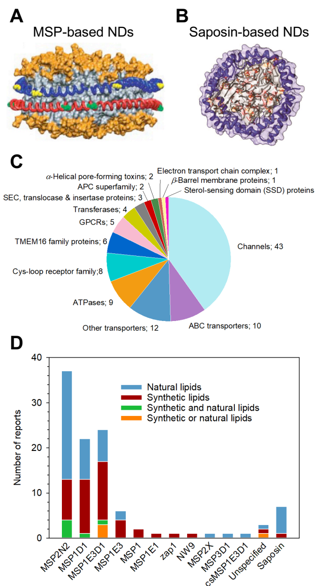
Figure 6. Membrane protein structures established in protein-based nanodiscs. (A) Molecular model of an MSP-based ND (side view). The two MSPs are shown in red and in blue, the 160 associated lipids in orange and grey. From (Shih et al., 2005). (B) Molecular model of a saposin-based ND (top view). The saposin A dimer is in purple, the 26 associated lipid molecules in reddish brown. From (Li et al., 2016). (C) Family distribution of MPs whose structures have been solved after reconstitution in protein-based NDs. “Other transporters” comprise cryo-EM structures of three multi-drug efflux transporters, three amino acid secondary transporters, and three transporters distributed among the three superfamilies of drug/metabolite transporters (DMT), CorA ion transporters and solute carrier (SLC) transporters. (D) Distribution of MSPs and lipids used to reconstitute MPs in protein-based NDs. The MSP called zap1 is derived from Zebra fish apo-lipoprotein A-1; MSP2X was constructed by linking two MSP1E3D1 chains with a two-amino acid linker; csMSP1E3D1 is a circularized version of MSP1E3D1. In three studies, the MSP used has not been clearly mentioned (“unspecified”). When the lipids were a mix of natural and synthetic lipids, they are noted as “natural and synthetic lipids”; when their nature has not been clearly mentioned, as “natural or synthetic lipids”.
