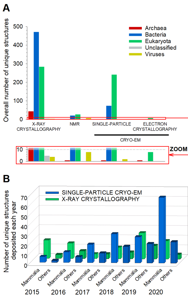
Figure 2. Distribution of unique MP structures according to biological origin. (A) Unique MP structures were classified into five groups (archaea, bacteria, eukaryotes, viruses and unclassified). The latter group comprises four crystallographic structures of de novo designed MPs. (B) Repartition of mammalian vs. other eukaryotic MP structures solved by either SP cryo-EM or X-ray crystallography over the past 6 years.
