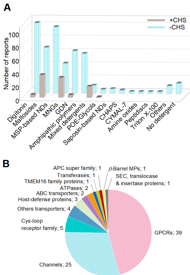
Figure 8. Addition of cholesteryl hemisuccinate (CHS) to MP samples. (A) Purification surfactants used in combination with CHS. (B) Distribution of MP structures solved in the presence of CHS among protein classes. “Others” are as described in the legend to Figure 7.
