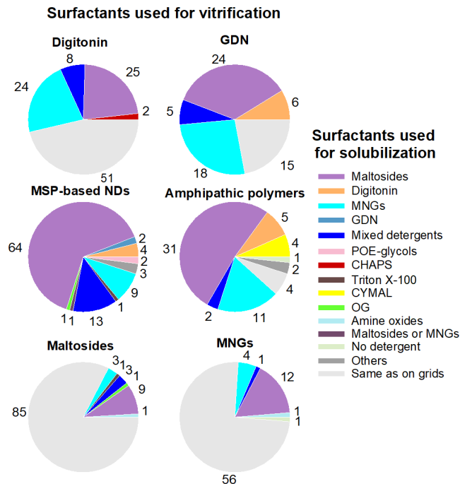
Figure 10. Surfactants used for solubilization and the initial steps of purification, depending on which surfactant was used for vitrification (either digitonin, GDN, MSP-based NDs, APols, maltoside detergents, or MNGs). All duplicates are included. In one case, the detergent used for vitrification has not been clearly specified and could be either maltosides or MNGs.
