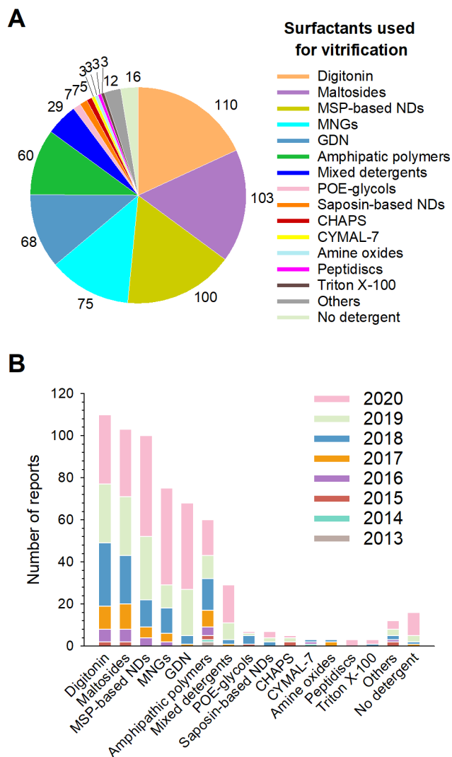
Figure 7. Surfactants used at the vitrification step. (A) Distribution of all surfactants in which MP structures have been solved by SP cryo-EM to a resolution \leq 5 \text{ \AA} (604 reports overall, taking all duplicates into account). (B) Number of near-atomic resolution MP structures reported each year since 2013 according to the type of surfactant used at the vitrification step. “Others” gather two cryo-EM structures obtained in Brij-35 and ten other structures obtained in one of the following surfactants: Tween 20, Igepal CA-630 (NP40), lauryldimethylamine oxide, MNA-C12, PCC-a-M, sodium cholate, Facade-EM (FA-3), octyl glucoside, sodium deoxycholate and liposomes. Sixteen of the cryo-EM structures gathered in Stephen White’s database are either MP fragments, toxins or peripheral MPs vitrified in the absence of detergent.
