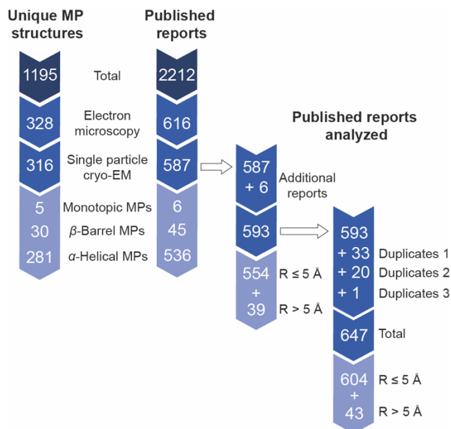
Figure 4. Number of unique cryo-EM MP structures and published reports analyzed in this study. Among the cryo-EM structures, SP analysis is the predominant technique, only nine unique MP structures having been solved using electron crystallography. Most cryo-EM MP structures have been solved by SP analysis applied to images of isolated MPs embedded in vitreous ice, one and two structures having been obtained by SP analysis applied to 2D crystals and helical assemblies, respectively. The list of reports analyzed comes from Stephen White’s database, manually completed with sixty SP cryo-EM structures for which a PDB and/or EMDB accession number was available (see below). Two cryo-EM structures of MPs reconstituted into liposomes have been included. In addition, examination of each of the 587 studies revealed that some cryo-EM structures were missing. They have been manually integrated into the list of reports as follows: a ) in four studies, an additional cryo-EM structure of a distinct MP or MP complex was identified and added to the list of reports, b ) in 50 studies, a 3D reconstruction of a MP has been obtained in two different surfactants, yielding two distinct refined structures, generating two sets of experimental conditions that have been included in our analysis as “duplicates”, and c ) in 2 studies, the cryo-EM structure of a MP has been obtained in three different surfactants, yielding “triplicates”. These additional experimental conditions were gathered in three groups: “Duplicates 1”: distinct cryo-EM structures were obtained in two (or three) different surfactants, whereas the detergent used for the purification was unchanged; “Duplicates 2”: both the purification and vitrification surfactants differed; “Duplicates 3”: the vitrification surfactant was the same but the purification was performed in two distinct detergents.
