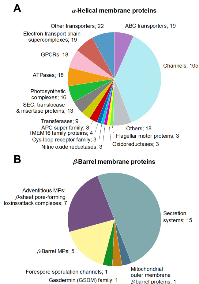
Figure 3. Family distribution of unique MP structures solved by SP cryo-EM. The groups of (A) \alpha -helical and (B) \beta -barrel MPs gather 281 and 30 unique MP structures, respectively. “Others”, in the \alpha -helical MP group, refers to cryo-EM structures of MPs belonging to the membrane-spanning 4-domain (MS4) family, antiporters, cellulose synthases, sterol-sensing domain (SDD) proteins, Type VII secretion systems, intramembrane proteases, adventitious MPs ( \alpha -helical pore-forming toxins), host-defense proteins, decarboxylases, novel receptors (STRA6 retinol-uptake receptor in complex with calmodulin), transhydrogenases, adenylyl cyclases, chain length determinant proteins and glycoproteins. “Other transporters” gather one cryo-EM structure of drug/metabolite transporter, two structures of H^+/Cl^- or F^- exchange transporters, two structures of transporters belonging to the major facilitator superfamily (MFS), three structures of multi-drug efflux transporters and, finally, fourteen structures of MPs belonging to the solute carrier (SLC) transporter superfamily.
