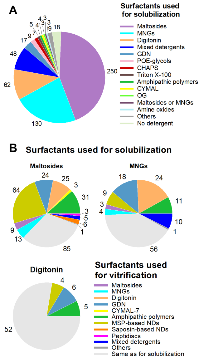
Figure 9. Surfactant exchange between MP purification and sample deposit onto cryo-EM grids. (A) Detergents used for MP solubilization and the initial steps of purification. In three cases (labeled “Maltoside or MNGs”), the detergent used for solubilization has not been clearly specified. (B) Surfactants used for vitrification, depending on which detergent was used for solubilization, namely either maltoside detergents (mainly DDM), MNGs (mainly LMNG), or digitonin. In Panel A, the analysis includes duplicates provided that the surfactants used for solubilization was different ( i.e. including duplicates 2 and 3), whereas in panel B all duplicates leading to \leq 5 Å structures have been included. References to studies using the combinations of surfactants shown in Fig. 9B are given in the S.I. in the legend to Table S1.
