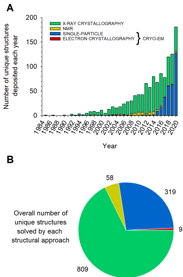
Figure 1. Distribution of unique MP structures solved by each structural approach between 1985 and January 1st, 2021. (A) Number of unique MP structures deposited each year using each approach. (B) Distribution of the 1195 unique structures extracted from Stephen White's database ( https://blanco.biomol.uci.edu/mpstruc/ ) according to the approach used to solve them. The figures were prepared using the January 8 th , 2021, update of MP structures from this database. Some MP structures published in 2020 may therefore not be included.
