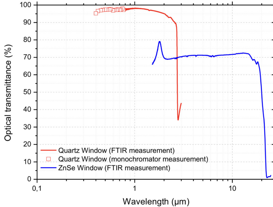
Figure 2. Optical Transmittances of quartz and ZnSe cryostat windows.
