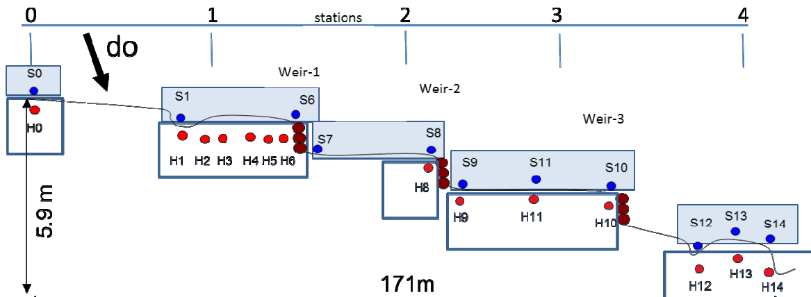
Fig.2: Longitudinal profile of the Chaudanne River around the CSOU and location of the sampling points
