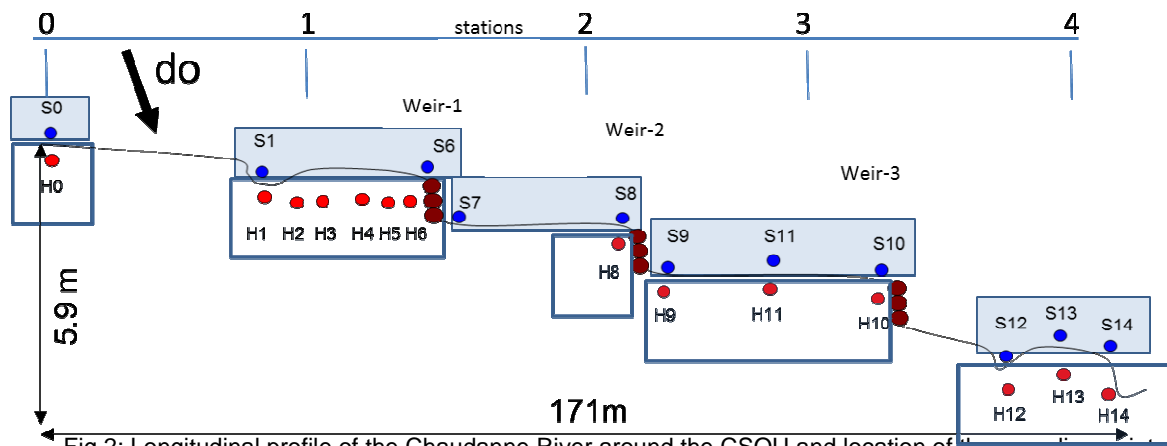
Fig.2: Longitudinal profile of the Chaudanne River around the CSOU and location of the sampling points
