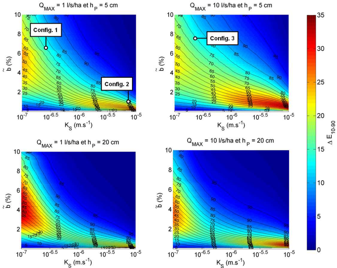
Figure 2 – Sizing diagrams for h_p = 5 and 20 cm and Q_{MAX} = 1 and 10 l/s/ha (contour lines = 10^{th} percentile of simulated efficiencies, \Delta E_{10-90} = difference between the 90^{th} and the 10^{th} percentile of simulate efficiencies)
