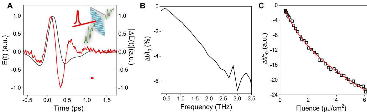
Figure 4: (A) The pulse transmitted through the composite HgTe film E(t) (left) and the difference of the THz electric field transmitted through the NCs with and without optical pumping, expressed as |\Delta E(t)| = |E_{\text{ON}}(t) - E_{\text{OFF}}(t)| (right). (B) Amplitude spectrum of the pump-induced change in transmission, \Delta t(\omega)/t_0(\omega) for a delay after the optical pump excitation of 2 ps and an incident pump fluence of 6 \mu\text{J cm}^{-2} . \Delta t(\omega) is the difference of the transmission with and without photoexcitation, \Delta t(\omega) = t_{\text{ON}}(\omega) - t_{\text{OFF}}(\omega) . (C) The peak amplitude of \Delta t/t_0 as a function of the incident optical pump fluence from 0.4 \mu\text{J cm}^{-2} to 6 \mu\text{J cm}^{-2} . The red line is a fit by a square root law.
