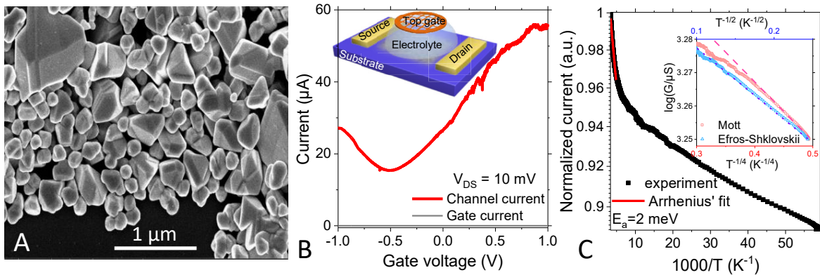
Figure 1: (A) Scanning electron microscopy image of large HgTe NCs. (B) Transfer curve (drain and gate current as a function of the applied gate bias) for a thin film made of large HgTe NCs used as the channel of an electrolytic transistor. Inset is a scheme of the field-effect transistor. (C) Current in logarithmic scale as a function of the temperature for a thin film made of large HgTe NCs. Arrhenius' fit of the curve in the vicinity of room temperature leads to an activation energy of 2 meV. The inset is a plot of the log of the current as a function of T^{-1/2} and T^{-1/4} .
