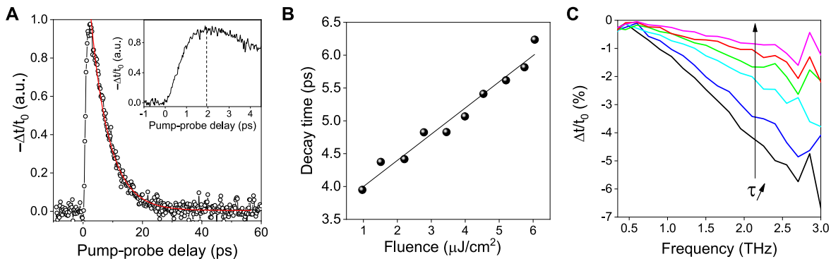
Figure 5: (A) The dynamics of the change of the transmission -\Delta t/t_0 as a function of the pump-probe delay time. (B) Decay time of -\Delta t/t_0 as a function of the incident optical pump fluence, showing a slow-down of the decay as the incident fluence is increased. (C) Frequency-dependent differential transmittance spectra \Delta t(\omega)/t_0(\omega) measured at different pump-probe delay times from 2 ps to 9 ps.
