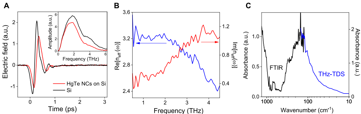
Figure 2: (A) The electric fields of the THz pulses transmitted through the HgTe composite film sample (red line) and through the Si substrate reference sample (black). Inset: corresponding amplitude spectra obtained by fast Fourier transform of the temporal traces. (B) The real and imaginary part of the effective index \tilde{n}_{\text{eff}}(\omega) of the composite film composed by the NCs and their surrounding environment is made of dodecanethiol ligands and air. (C) Absorbance spectra from 1330 \text{ cm}^{-1} to 10 \text{ cm}^{-1} of the HgTe sample obtained by THz TDS (blue line) and FTIR (black line) measurements. The FTIR data are arbitrarily matched to the TDS one in their overlapping spectral region, as measurements were performed independently.
