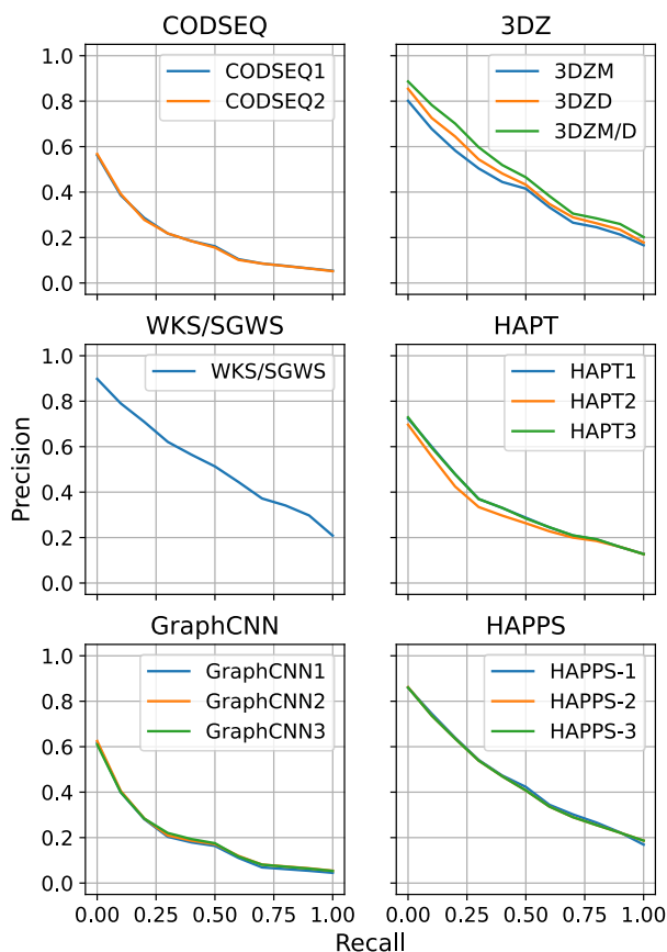
Fig. 5. Precision-Recall curves at the species level.
