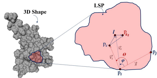
Fig. 3. Local Surface Patch (LSP), P_i with pairwise points (p_i, p_j) as part of a surflet-pair relation for (p_i, n_i) and (p_j, n_j) , with p_i being the origin. \theta and \phi are the angles of vectors projection about the origin, p_i . \theta is the projection angle from vector \langle p_i - p_j \rangle to vector \langle p_i - p_c \rangle while \phi is the projection angle from vector \langle p_i - p_j \rangle to vector \langle p_i - l \rangle . The LSP centre is given by p_c , keypoint is given as p_{k_i} where i = 2 . Finally, l is the vector position of p_{k_i} - p_c .
