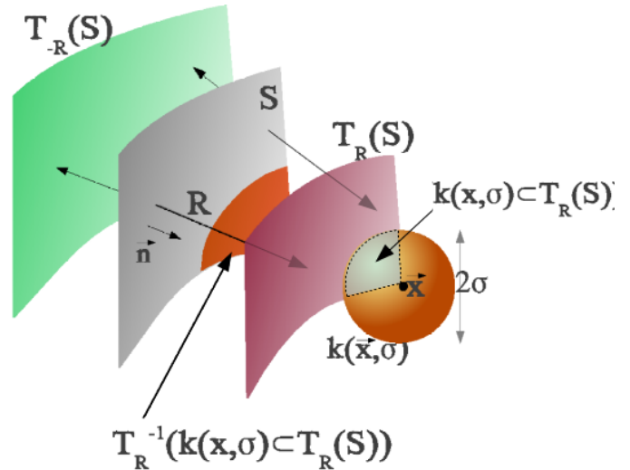
Fig. 1. APT measures the area of the part of the input surface that, projected along the normal at a selected distance, is included in a circular neighborhood of the point of interest (see subsection 4.4).
