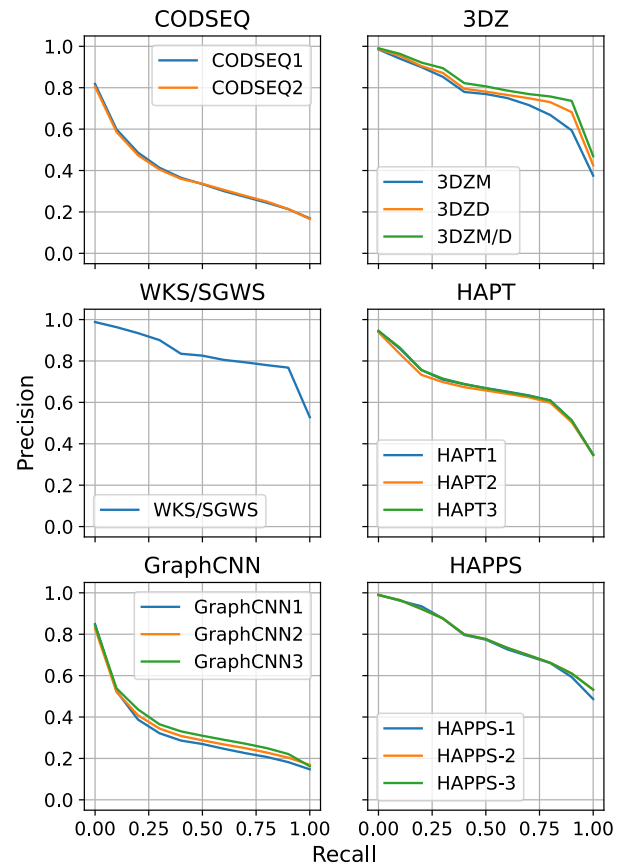
Fig. 4. Precision-Recall curves at the protein level.
