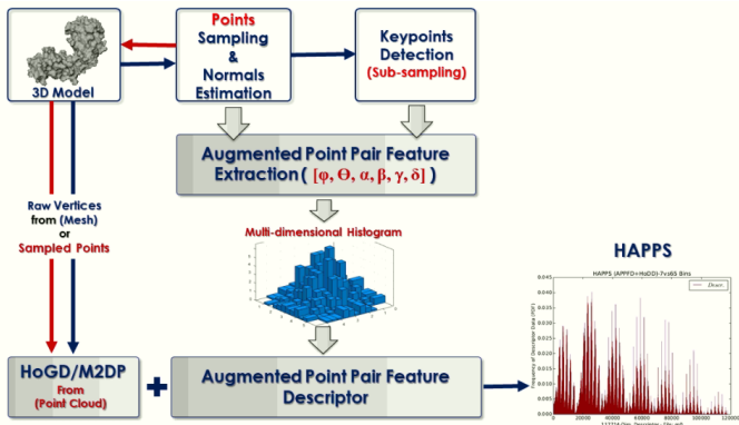
Fig. 2. Overview of HAPPS algorithm.
