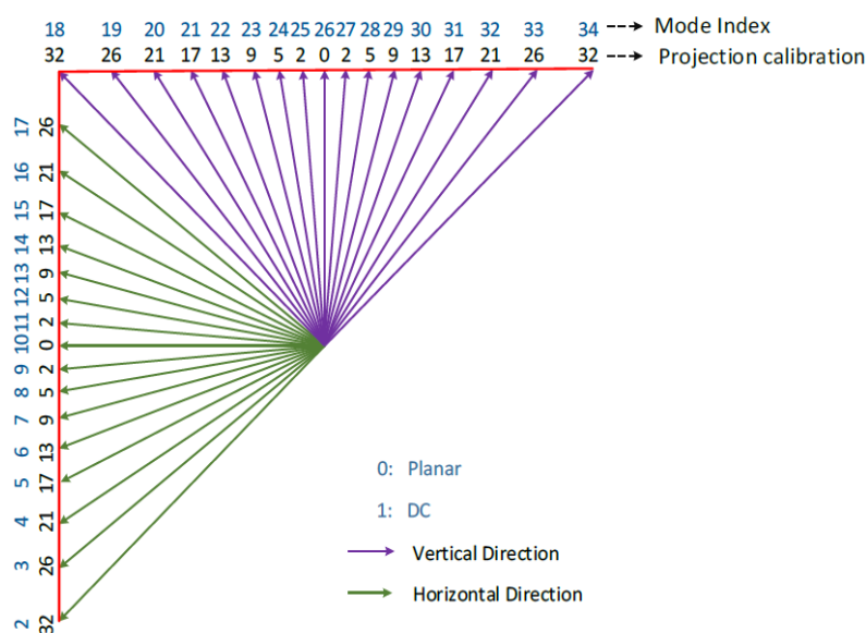
Figure 11. Intra-prediction modes in High-efficiency video coding (HEVC) [29].
