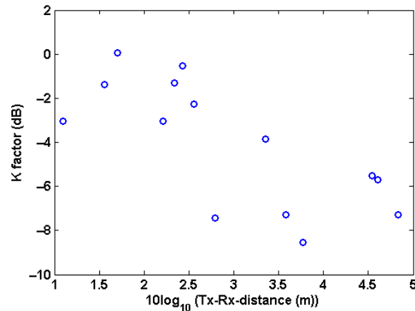
Figure 8. Measured K-factor.
