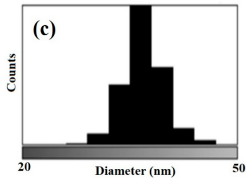
Figure 5. (a) 40° tilted view SEM image of perpendicular ZnO NWs arrays grown on ZnO SL/Si (100) substrates at 10 mTorr, (b) top view SEM image of the as-grown ZnO NWs, (c) corresponding size distribution histogram of the ZnO NWs arrays.
