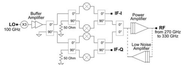
Fig. 3. Schematic of the active electronic transmitter and receiver MMIC. The two components integrate a frequency multiplier by three, a buffer amplifier, a fundamental passive I/Q mixer, and a final amplifier for the transmitter and a low noise amplifier for the receiver. The MMICs are packaged in a waveguide split-block module.
