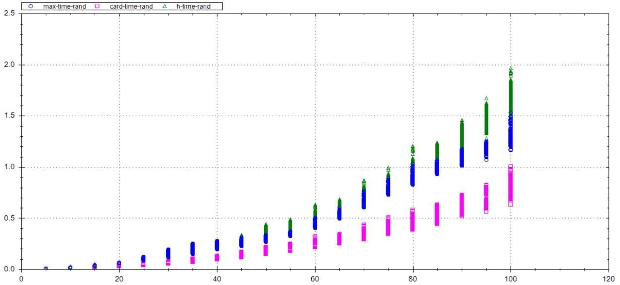
Figure 15: Time on Sophia Antipolis dataset when arguments are attributed random basic weights. The x axis shows the number of arguments in thousands . The y axis shows the time in thousands of seconds.
