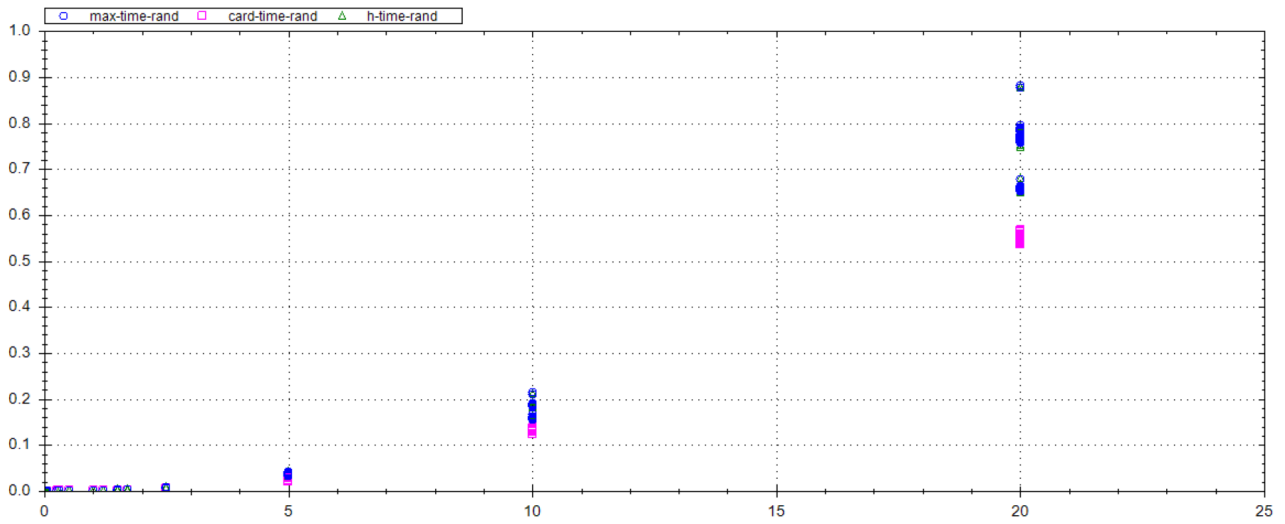
Figure 9: Time on Barabási-Albert dataset when arguments are attributed random initial weights . The x axis shows the number of arguments in thousands . The y axis shows the time in thousands of seconds.
