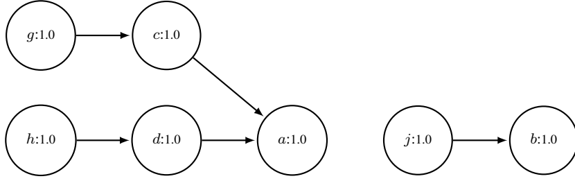
Figure 4: Weighted graph \mathbf{G}_4
