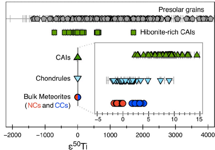
Fig. 1 Variation in ^{50}\text{Ti}/^{47}\text{Ti} , expressed in \epsilon units (parts per 10,000; see Sect. 3 for details), in presolar grains, CAIs, chondrules, and “bulk” CC- and NC-type meteorites (chondrites and achondrites). The inset illustrates that CAIs, chondrules, and bulk meteorites record small \epsilon^{50}\text{Ti} variations ( <20 \epsilon units) compared to presolar grains ( \geq 5000 \epsilon units, corresponding to 500 ‰ in \delta units). Error bars are smaller than symbol sizes in most cases, except for presolar grains. Modified from Torrano et al. (2019) with data from the literature (Alexander and Nittler 1999; Amari et al. 2001; Davis et al. 2018; Gerber et al. 2017; Gyngard et al. 2018; Hoppe et al. 1994; Huss and Smith 2007; Ireland et al. 1991; Kööp et al. 2016; Niemeyer 1988; Render et al. 2019; Torrano et al. 2019; Trinquier et al. 2009; Zhang et al. 2012; Zinner et al. 2007).
