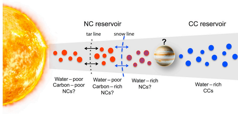
Fig. 4 Schematic cross-section of the protoplanetary disk (not to scale). Planetesimals with NC- and CC-type nucleosynthetic compositions are represented in red and blue, respectively. The two reservoirs are considered to have been spatially separated (e.g., Warren 2011), possibly as a result of the early accretion of proto-Jupiter (Kruijer et al. 2017). Based on the radial gradient in temperature, planetesimals that accreted beyond the snow line (where T \approx 160 K at the midplane; Hayashi 1981; Lodders 2004) are expected to be water-rich, whereas ‘dry’ (i.e., ice-free) planetesimals that formed between the tar- and snow line could have incorporated refractory organics (Lodders 2004; Nakano et al. 2020). The radial position of the mobile condensation fronts relative to the Jupiter barrier likely played a fundamental role in the distribution and transport of inorganic ices (and organics) in the disk during the first few million years of solar system history.
