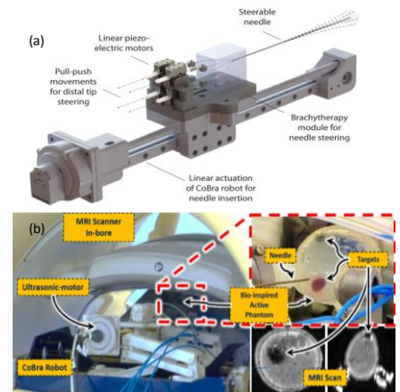
Figure 1: (a) Steerable needle module; (b) CoBra robot and active prostate phantom
