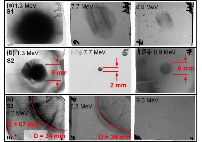
FIG. 2. Images of RCF for (a) unfocused protons in the S1 (30 mm) position, (b) focused protons in the S2 (30 mm) position, and (c) focused protons in the S3 (0.56 m) position. The energies marked on the films correspond to the average proton energy incident on the layer. All films are plotted with the same spatial scale, but have different gray-scales.
