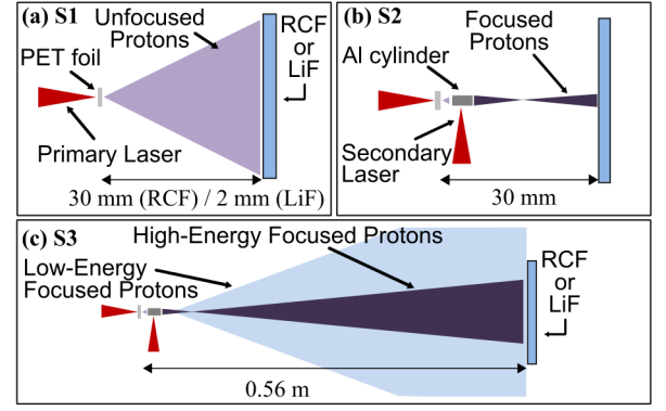
FIG. 1. Diagrams of the different setups used in this study: (a) S1: the broadband, unfocused proton beam, (b) S2: proton focusing using the micro-lens, irradiated by the secondary beam, and (c) S3: focused protons at longer distances, where the higher divergence of the lower-energy protons decreases their contribution to the measured spectrum.
