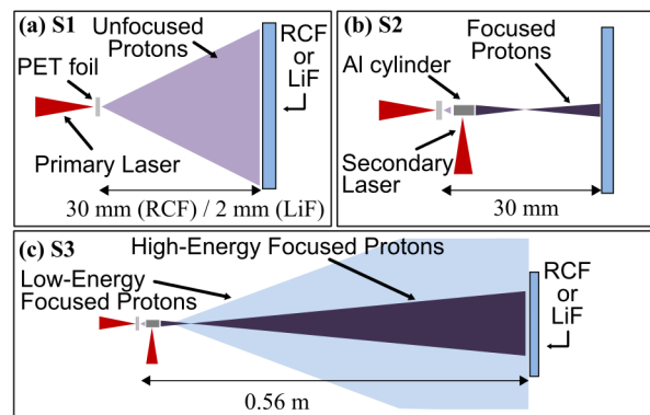
FIG. 1. Diagrams of the different setups used in this study: (a) S1: the broadband, unfocused proton beam, (b) S2: proton focusing using the micro-lens, irradiated by the secondary beam, and (c) S3: focused protons at longer distances, where the higher divergence of the lower-energy protons decreases their contribution to the measured spectrum.
