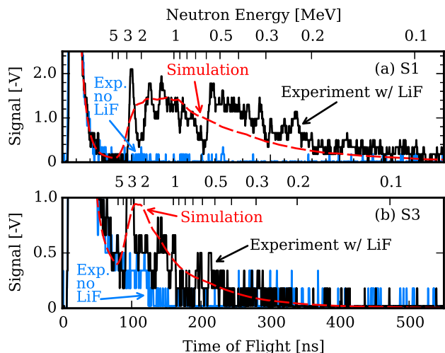
FIG. 4. Plot of the ntof traces from the experimental data without neutron production (light lines), with neutron production (dark lines) and the simulated neutron signal (dashed lines). Time zero corresponds to the arrival of the laser. The plots (a) and (b) refer to setups S1 and S3, respectively.
