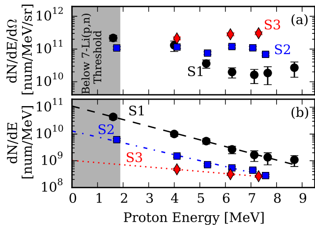
FIG. 3. Measured single-shot energy-spectra of the proton fluence from S1 (circles), S2 (squares) and S3 (diamonds). Error bars for S1 represent variation across multiple shots, whereas S2 and S3 are single shots with 10% film batch variability uncertainty. The top plot shows the average fluence which is determined by dividing the total signal on the film by the solid angle subtended by the signal. The bottom plot shows the total number of protons hitting the film stack, where lines show exponential fits to the spectra, dN/dE = (N/T)e^{-E/T} . Where N is 1.9 \times 10^{11} , 2.5 \times 10^{10} and 5.5 \times 10^9 , and T is 1.72, 1.96 and 5.32 MeV for the S1, S2 and S3 cases, respectively.
