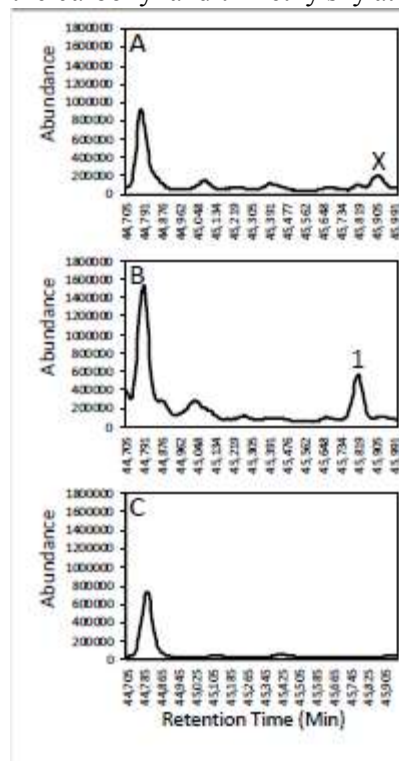
Figure 4: Mass spectra and drawings representing fragmentation scenarios for 12,13-dihydroxy-octadec- cis -9-enoic acid methylated on carboxyl and silylated on hydroxyls.
