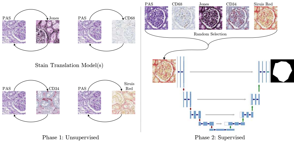
Figure 3: Overall diagram of the proposed approach. Phase 1, translation models are learnt to translate images from the source domain to the target domains; Phase 2, patches of the source domain are randomly translated to the target domains during training (U-Net image taken from [37]).
