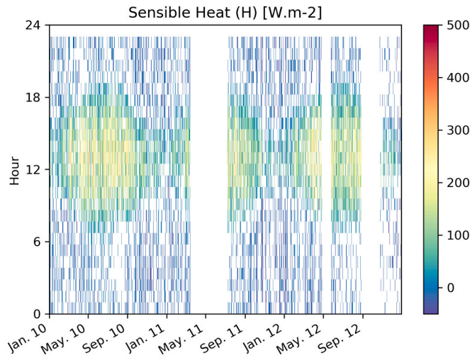
Fig. 4. Heatmap of daily and hourly variations of Sensible Heat (H) calculated by the Eddy Covariance method. Unavailability of valid data is represented by the white color.
