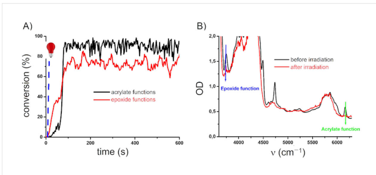
Figure 4: A) Photopolymerization profiles of PETIA/epoxy blend 1:1, w/w under air (acrylate and epoxy functions conversion vs irradiation time) in the presence of Cb /iod 0.3:2, w/w upon exposure to a laser diode at 785 nm ( 0.9 \text{ W/cm}^2 ), thickness = 1.4 mm. The irradiation starts at t = 10\text{ s} . B) FTIR spectra before and after irradiation.
