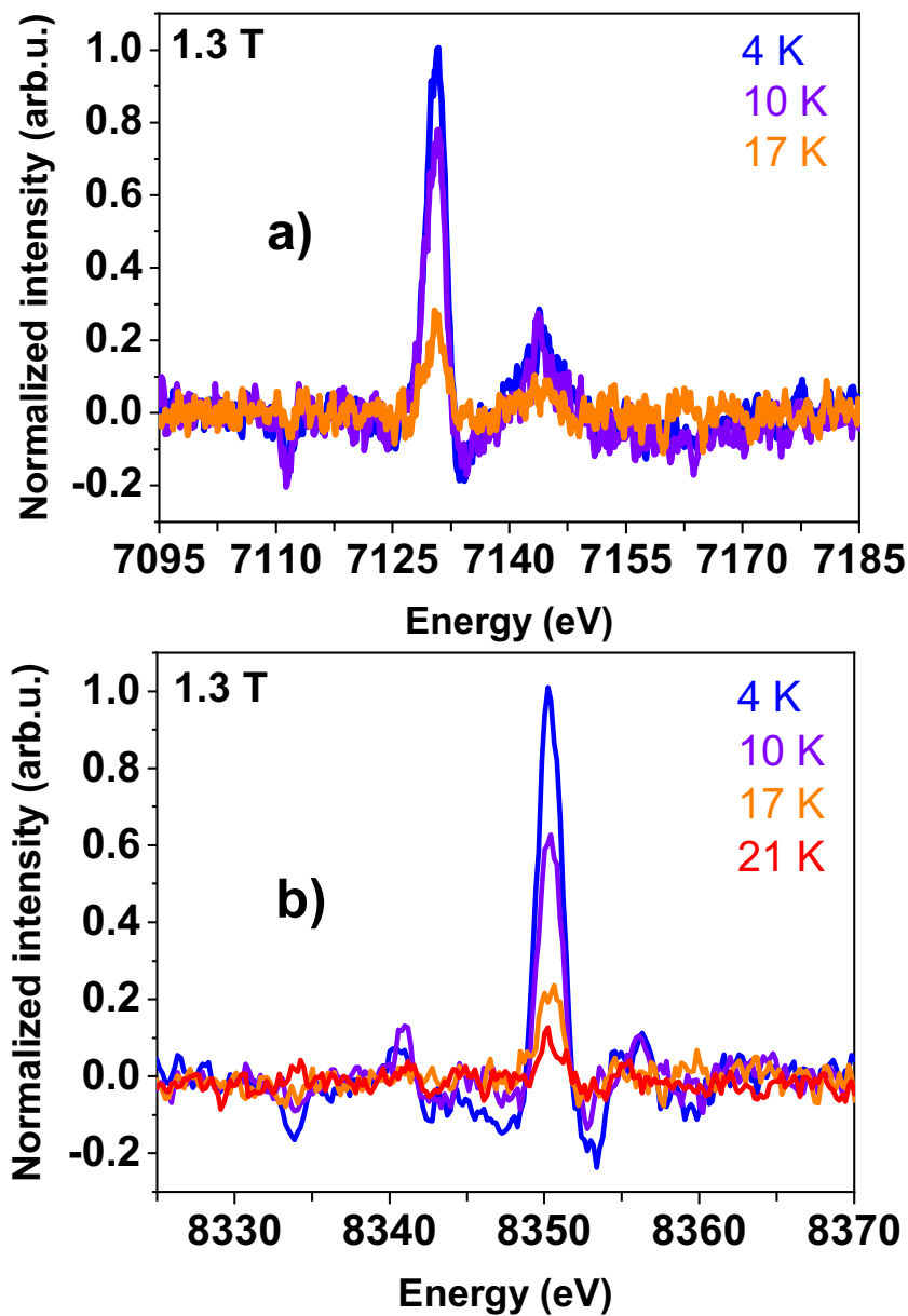
Fig. 2. Normalized (a) Fe and (b) Ni K-edges XMCD signals of NiFe recorded at 1.3 T for a variable temperature.
