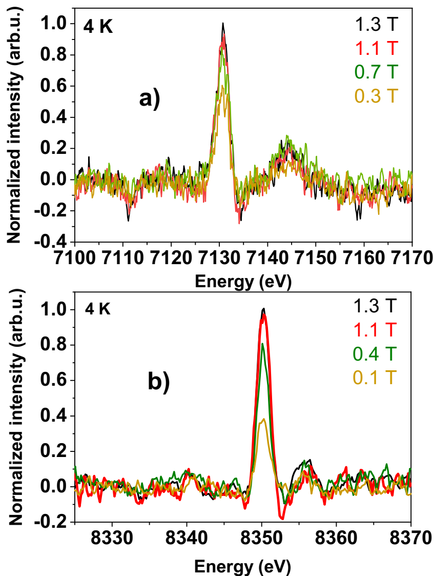
Fig. 4. Normalized (a) Fe and (b) Ni K-edges XMCD signals of NiFe recorded at 4 K for a decreasing variable magnetic field.
