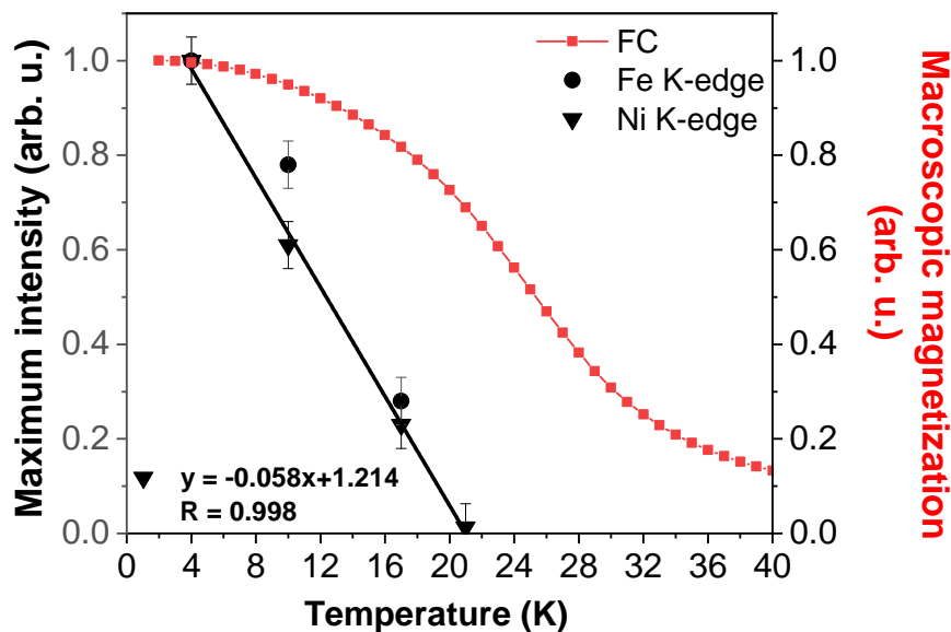
Fig. 3. Evolution for NiFe of the maximum intensity of the XMCD signals as a function of the temperature at both Fe (circles) and Ni (triangles) K-edges along with the macroscopic magnetization recorded by SQUID magnetometry (red curve). All the data were recorded for a 1.3 T magnetic field. The macroscopic magnetization at 4 K ( 47.4 \cdot 10^3 \text{ emu} \cdot \text{mol}^{-1} ) was renormalized so that the value is also set to 1.
