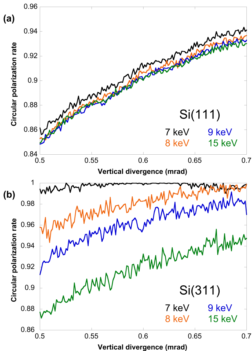
Fig. 7. Calculated circular polarization rate at the sample position for the 7-9 keV energy range (TM K-edges) and at 15 keV in the case of (a) the Si(111) polychromator and (b) the Si(311) polychromator.
