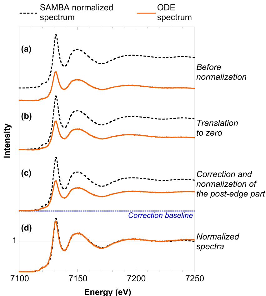
Fig. 1. Normalization procedure of the XANES spectrum recorded on ODE in the dispersive setup using the normalized EXAFS spectrum recorded on SAMBA in the conventional scanning mode for the example of CoFe at the Fe K-edge. From top to bottom (a) Before the normalization of the ODE spectrum, (b) Pre-edge part adjustment, (c) Post-edge part normalization, (d) After the full normalization procedure for the ODE spectrum.
