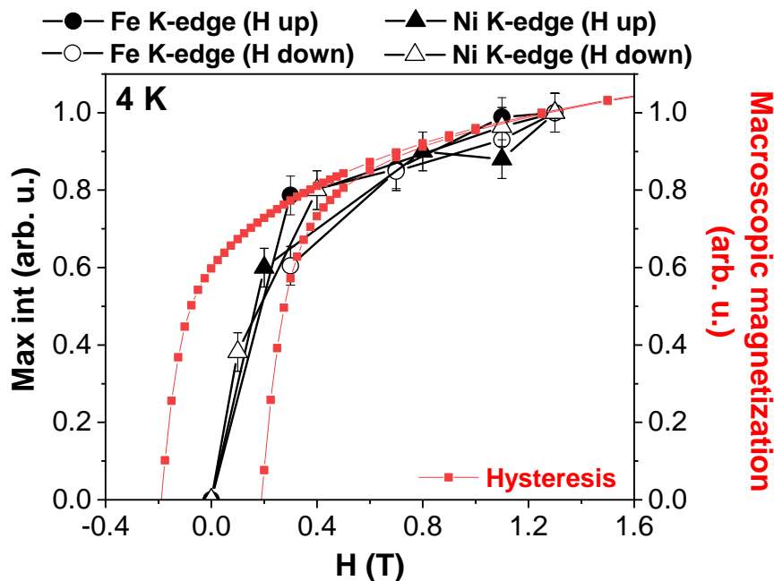
Fig. 5. Evolution for NiFe of the maximum intensity of the XMCD signals as a function of the applied external magnetic field at the Fe (circle symbols) and Ni (triangle symbols) for an increasing (black symbols) and decreasing (white symbols) magnetic field, compared with the macroscopic magnetization recorded by SQUID magnetometry (red line). The macroscopic magnetization at 1.3 T ( 47.4 \cdot 10^3 \text{ emu} \cdot \text{mol}^{-1} ) was renormalized so that the value is also set to 1.
