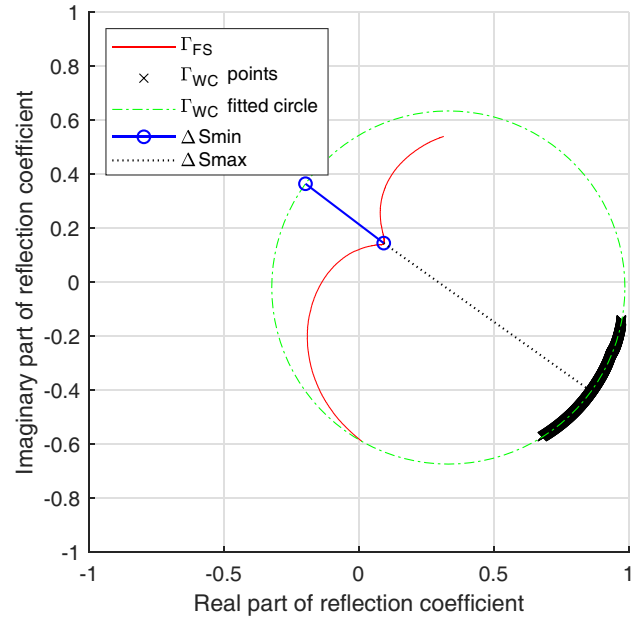
Figure 5. Reflection coefficient of the antenna in free space ( \Gamma_{FS} ) and Wheeler Cap ( \Gamma_{WC} ) with respect to complex load (case 2).
