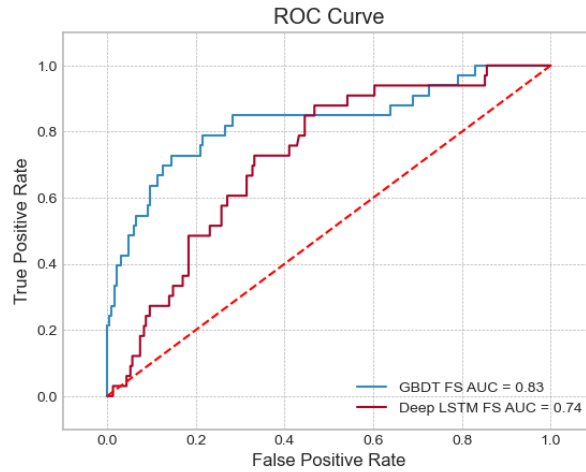
Fig. 2. ROC Curve of the two best models
