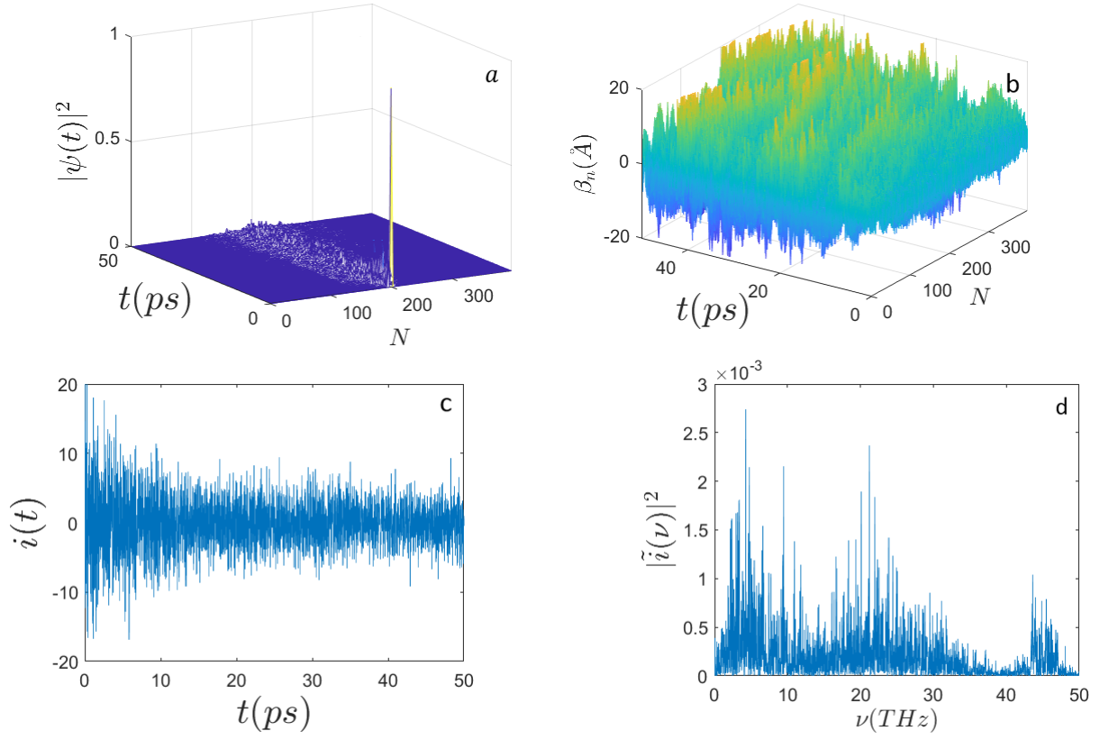
Figure 4: Time evolution of: a) the electron probability amplitude |\Psi(t)|^2 ; b) the average displacements \beta_n(\text{\AA}) ; c) the electron current i(t) (expressed in \mu\text{biot} ); d) the frequency spectrum |\tilde{i}(\nu)|^2 along the sequence of N = 398 nucleotides with the initial condition E_0 = 0.46 eV ( E' = 70 ). The initial electron excitation is peaked around the site n_0 = N/2 . The other parameters are the same of Fig. 1.
