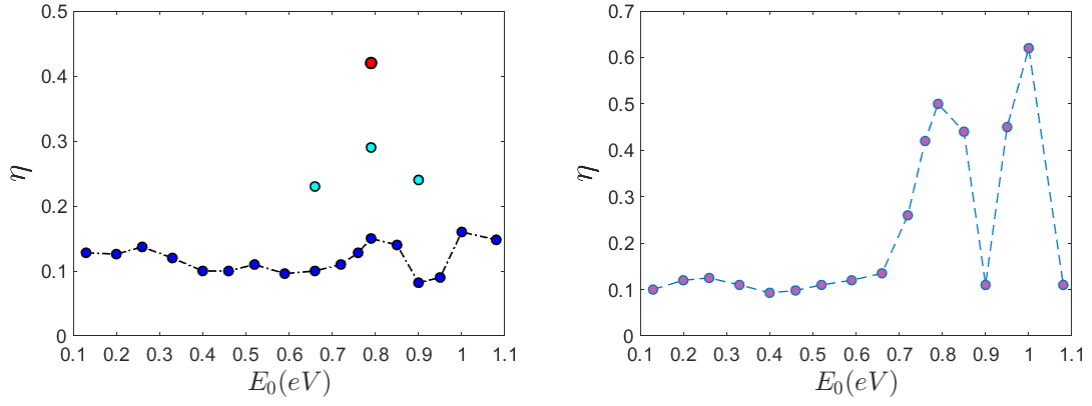
Figure 9: The normalized spectral entropy \eta versus the initial energy E_0 for a DNA protein. The parameters are the same of those reported for Fig. 1. The left panel refers to N = 398 bp where the dark blue circles correspond to the initial electron excitation peaked around the site n_0 = N/2 , the light blue circles correspond to n_0 = N/3 , and the red circle correspond to n_0 = 2N/3 . The right panel refers to N = 66 bp and the initial electron excitation is peaked around the site n_0 = N/2 .
