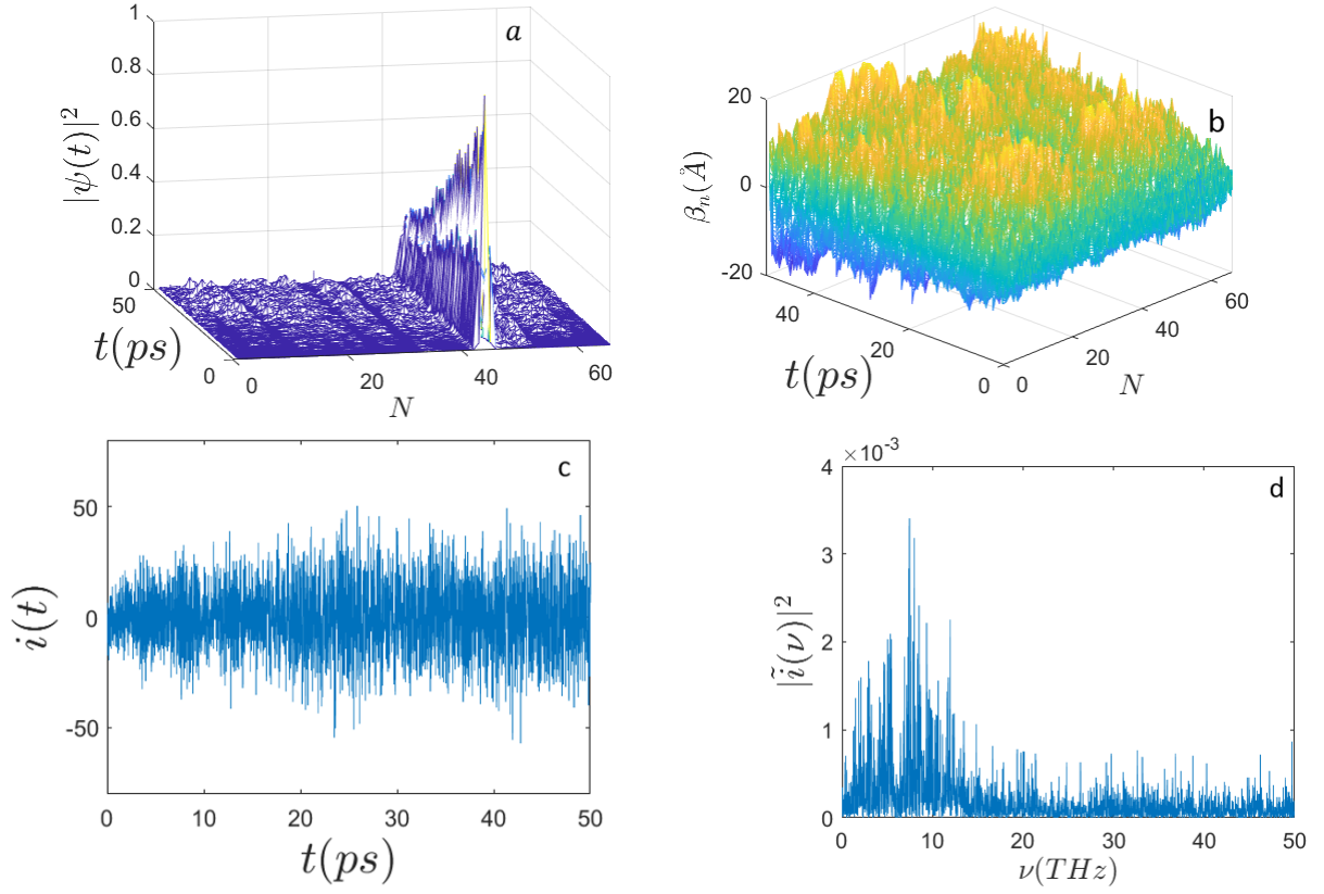
Figure 8: Time evolution of: a) the electron probability amplitude |\Psi(t)|^2 ; b) the average displacements \beta_n(\text{\AA}) ; c) the electron current i(t) (expressed in \mu\text{biot} ); d) the frequency spectrum |\tilde{i}(\nu)|^2 along the sequence of N = 66 nucleotides with the initial conditions E_0 = 0.9 eV ( E' = 136.7 ) and the initial electron excitation peaked around the site n_0 = 2N/3 . The other parameters are the same of Fig. 1.
