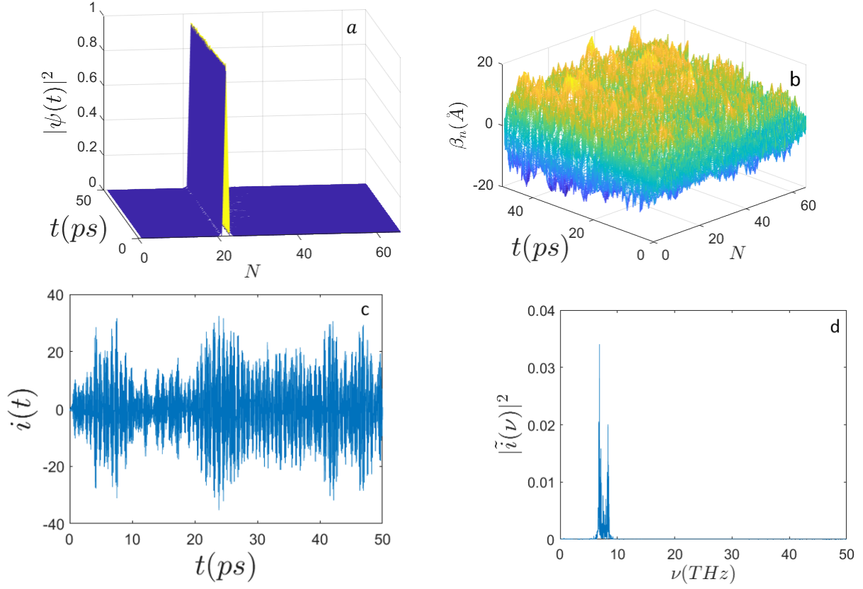
Figure 5: Time evolution of: a) the electron probability amplitude |\Psi(t)|^2 ; b) the average displacements \beta_n(\text{\AA}) ; c) the electron current i(t) (expressed in \mu\text{biot} ); d) the frequency spectrum |\tilde{i}(\nu)|^2 along the sequence of N = 66 nucleotides with the initial conditions E_0 = 0.2 eV ( E' = 30 ) and the initial electron excitation peaked around the site n_0 = N/3 . The other parameters are the same of Fig.1.
