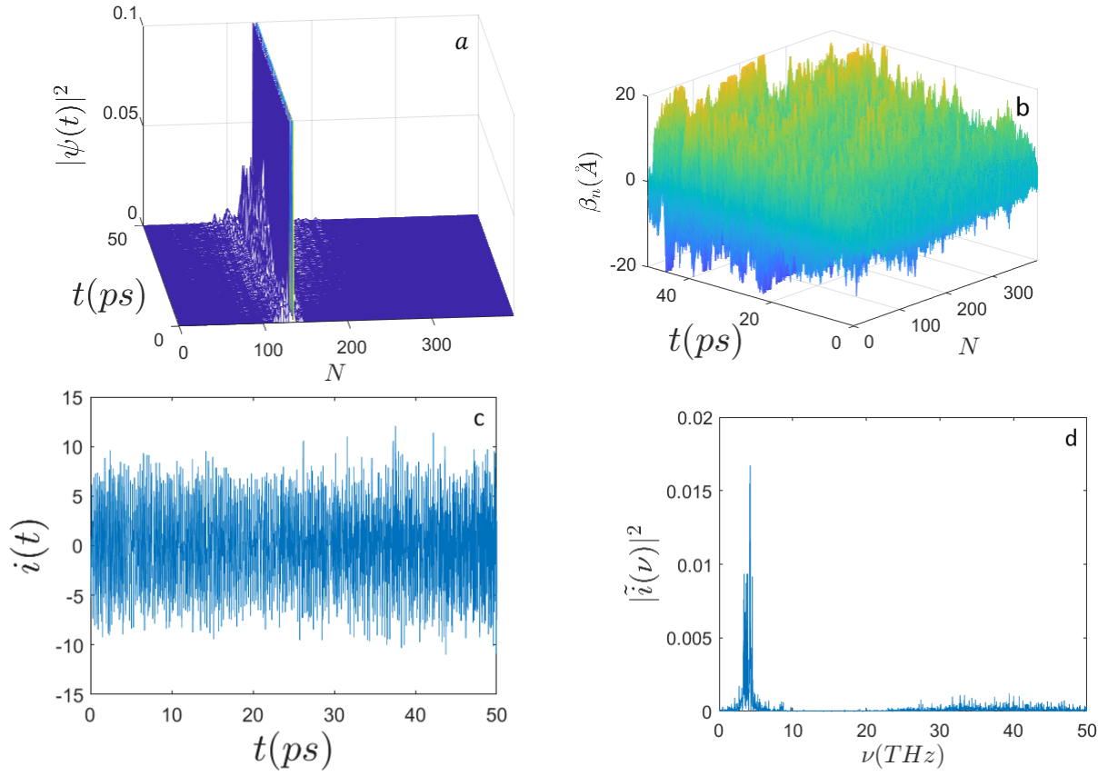
Figure 2: Time evolution of: a) the electron probability amplitude |\Psi(t)|^2 ; b) the average displacements \beta_n(\text{Å}) ; c) the electron current i(t) (expressed in \mu\text{biot} ); d) the frequency spectrum |\tilde{i}(\nu)|^2 along the sequence of N = 398 nucleotides. Initial conditions and parameters are the same of Fig. 1 but the initial electron excitation is peaked around the site n_0 = N/3 .
