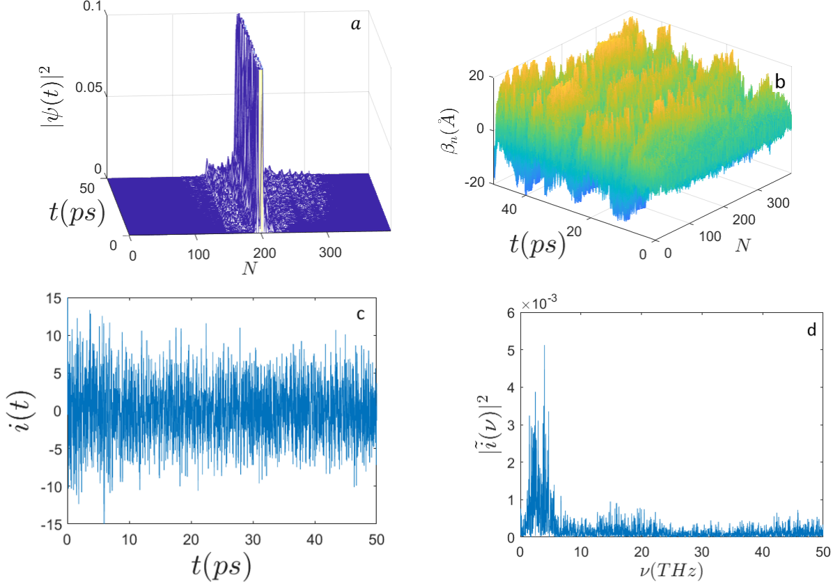
Figure 1: Time evolution of: a) the electron probability amplitude |\Psi(t)|^2 ; b) the average displacements \beta_n(\text{Å}) ; c) the electron current i(t) (expressed in \mu\text{biot} ); d) the frequency spectrum |\tilde{i}(\nu)|^2 along the sequence of N = 398 nucleotides. Initial conditions: T = 310^\circ\text{K} , n_0 = N/2 , E' = 100 , \epsilon' = 5 , \Omega' = 0.25 , \mu' = 0.5 , \sigma_0 = 0.1 , and the site-dependent parameters J'_n , and \chi'_n corresponding to E_0 = 0.658 eV, \epsilon = 0.0329 eV, \Omega_n = V^2 M_n / a^2 , J_n , and \chi_n in Eqs. (22) and (23), respectively. Initial electron excitation peaked around the site n_0 = N/2 .
