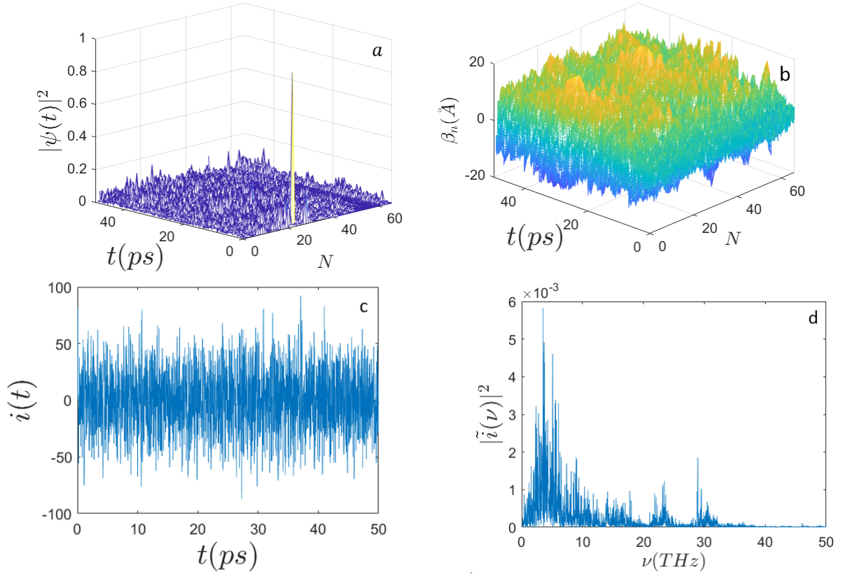
Figure 6: Time evolution of: a) the electron probability amplitude |\Psi(t)|^2 ; b) the average displacements \beta_n(\text{\AA}) ; c) the electron current i(t) (expressed in \mu\text{biot} ); d) the frequency spectrum |\tilde{i}(\nu)|^2 along the sequence of N = 66 nucleotides with the initial conditions E_0 = 0.79 eV ( E' = 120 ) and the initial electron excitation peaked around the site n_0 = N/3 . The other parameters are the same of Fig. 1.
