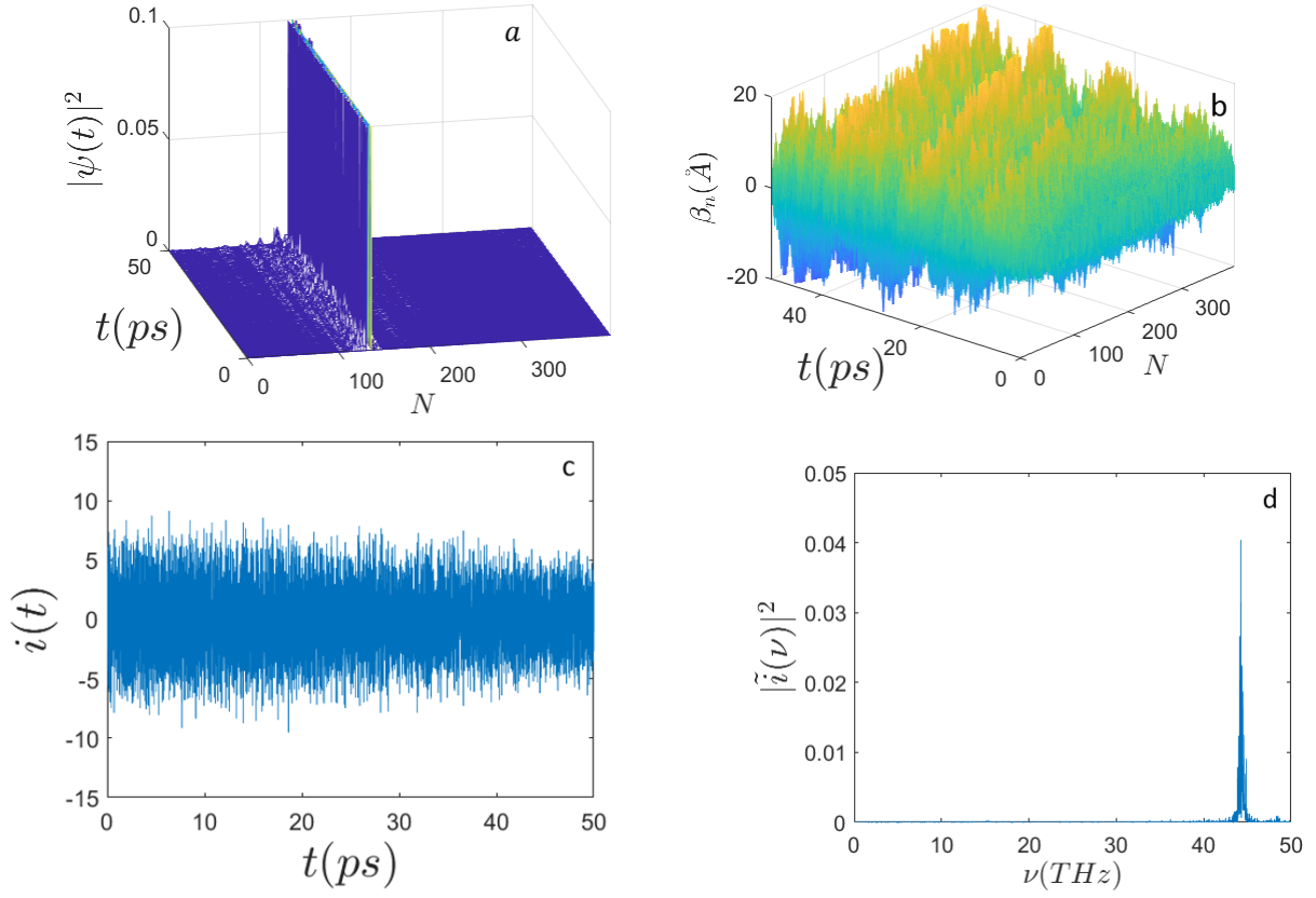
Figure 3: Time evolution of: a) the electron probability amplitude |\Psi(t)|^2 ; b) the average displacements \beta_n(\text{\AA}) ; c) the electron current i(t) (expressed in \mu\text{biot} ); d) the frequency spectrum |\tilde{i}(\nu)|^2 along the sequence of N = 398 nucleotides, with the initial condition E_0 = 0.79 eV ( E' = 120 ) and the initial electron excitation peaked around the site n_0 = N/3 . The other parameters are the same of Fig. 1.
