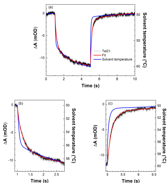
Figure 5: (a) \Delta A (black lines) measured at 293 nm, for Tel21 with 150 mM Na + , following a T-jump of 10 ^{\circ}\text{C} after 1 s, for T_{\text{ini}} = 50^{\circ}\text{C} , and a subsequent cooling down to the initial temperature after 5 s, (b) \Delta A observed during 1.5 s after the T-jump and (c) after the cooling down. Blue lines correspond to the simulation of the solvent temperature change. Red lines correspond to the fits
