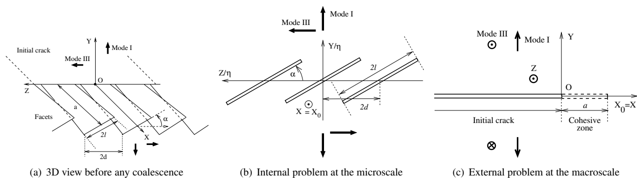
Figure 2: Sketch and notations of the initial crack and the facet formation: decomposition of the initial 3D problem (a) in two 2D problems: at the microscale (obtained by rescaling X and Y axis by X/\eta and Y/\eta , with \eta \equiv d/a \rightarrow 0 ), the facets appear as an array of parallel echelon cracks subjected to remote stresses (b); at the macroscale, they are embedded in a cohesive zone (c).
