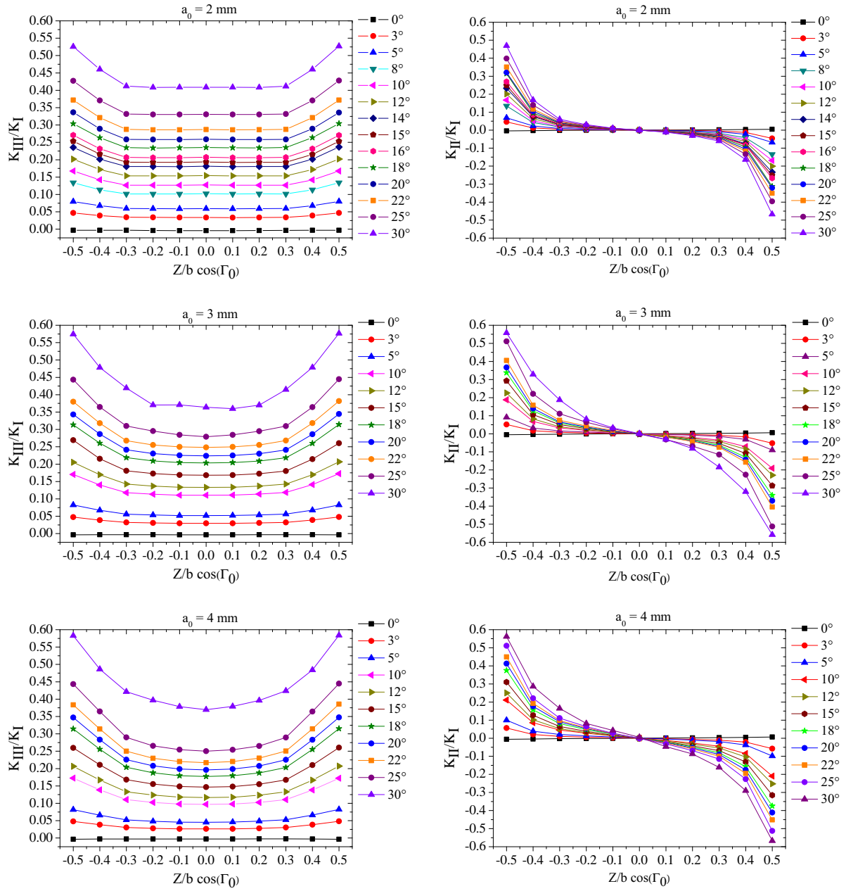
Figure C.12: Evolution of the ratio K_{II}/K_I and K_{III}/K_I along the crack front as calculated by Finite Elements.
