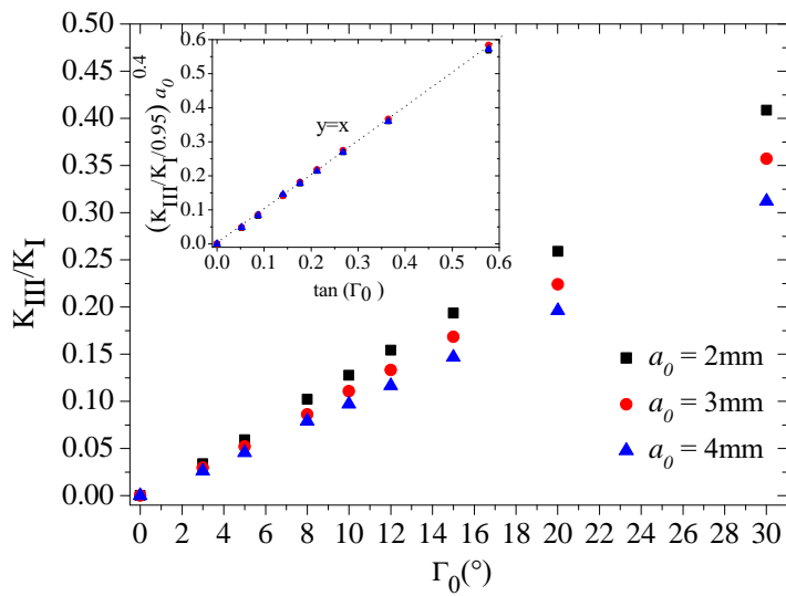
Figure C.13: Ratio of the mode III over the mode I SIF taken at the middle of the crack front. Inset: the dependance with a_0 and \Gamma_0 can be encompassed in the single formula (9).
