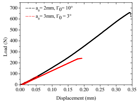
(c) Typical loading curve
