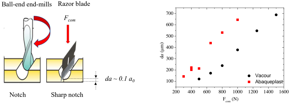
Figure B.10: Left: Notch milling and sharp notch formation. Right: Length of the additional precrack as a function of the compressive applied force for the two brands of PMMA (Vacour and Abaqueplast) used in this study.
