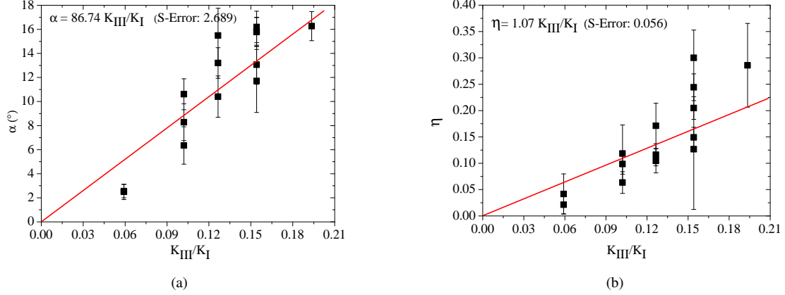
Figure 7: (a) The tilt angle \alpha is taken as the maximum value of \alpha(a) (blue dot in Fig. 6b), the error bars corresponds to the standard deviation of the facet angle distribution at the peak location. (b) The coarsening rate \eta is taken as the slop of the linear part of the evolution d(a) (in blue in Fig. 6c), the error bars corresponds to the upper and lower bounds of the 95 % confidence interval of the linear regression.
