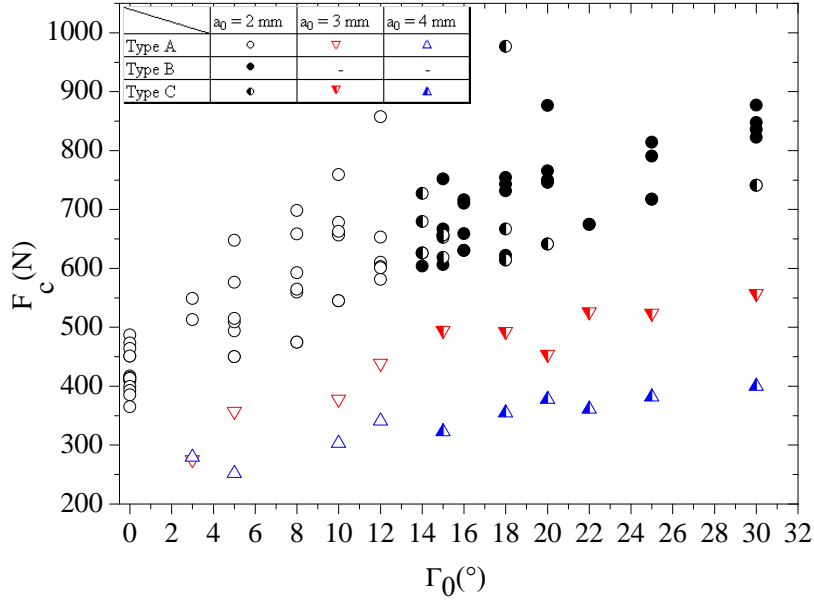
Figure 4: Maximum load F_c measured for several values of \Gamma_0 and a_0 .
