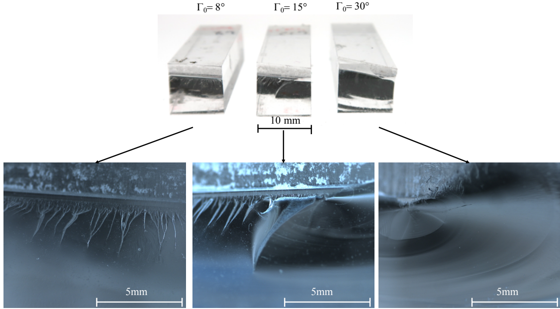
Figure 5: Fracture surfaces as observed by numerical microscopy. \Gamma_0 = 8^\circ corresponds to Type A, for \Gamma_0 = 15^\circ to Type C, for \Gamma_0 = 30^\circ to Type B.
