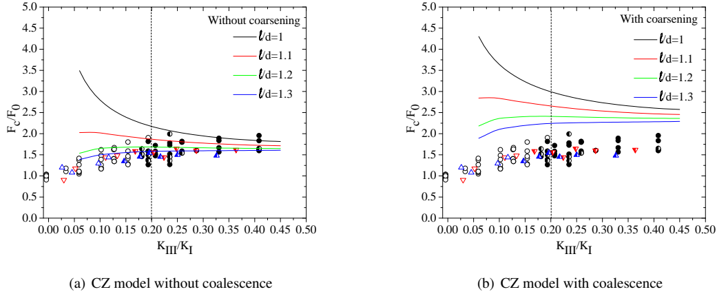
Figure 8: Comparison between the CZ model and the experimental values of F_c/F_0 . The point symbols are the same than on Fig. 4. The CZ model is applicable only for type A fracture surfaces (empty symbols) that is on the left of vertical line located around K_{III}/K_I \sim 0.2 .
