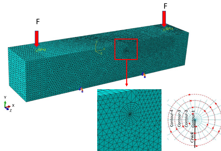
Figure C.11: Meshing used in the Finite Element model with the imposed Boundary Conditions
