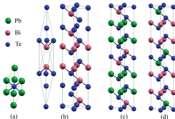
Figure 1 (a) Primitive cell of PbTe; (b) primitive and conventional cells of \text{Bi}_2\text{Te}_3 ; (c) 1 \times 1 \times 2 supercell of \text{Pb}_2\text{Bi}_2\text{Te}_5 in stacking A; (d) 1 \times 1 \times 2 supercell of \text{Pb}_2\text{Bi}_2\text{Te}_5 in stacking B.
