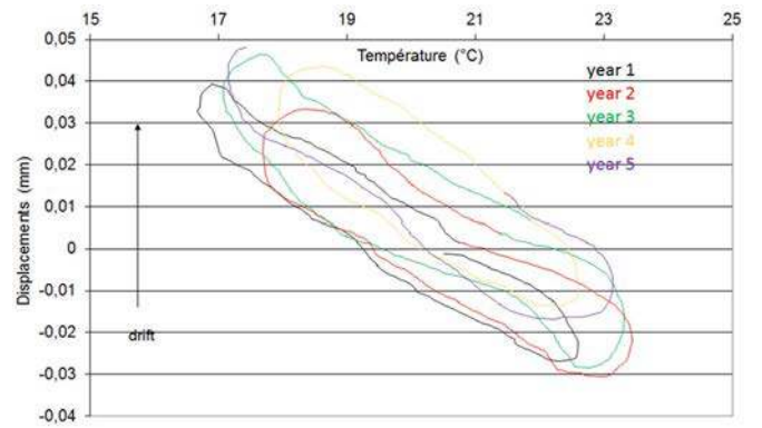
Fig. 9. –Length variation versus temperature for the D1–6 m depth extensometer– Colour change each July 22nd that is one year of recording. The resolution of the extensometer is less than 0.01 mm.
