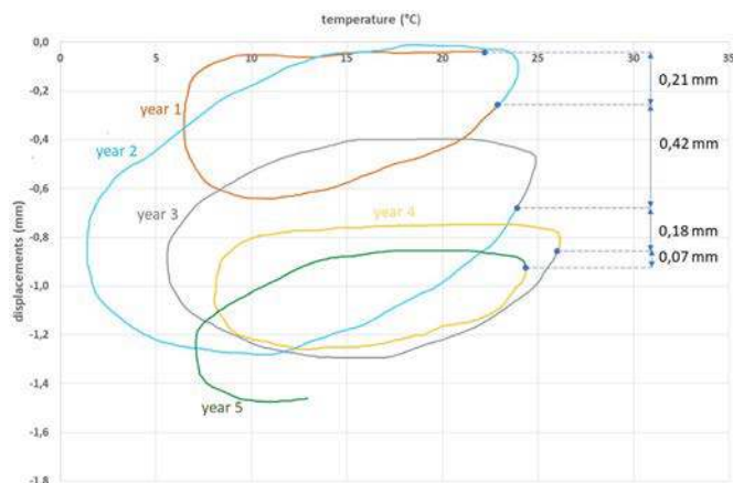
Fig. 8. – Correlation between length variation and temperature on F2.
