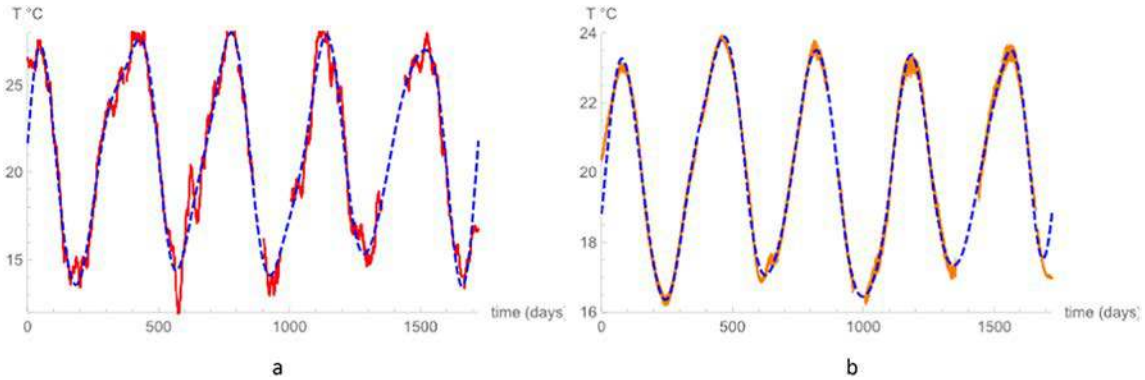
Fig. 7. - Temperatures measured in D1 a -Red line at two metres depth, b - Orange Line at six metres depth. Blue dashed line: Temperature estimated with Fourier series decomposition (please note the temperature scale is different on the 2 graphs to better show the adjustment). (For interpretation of the references to colour in this figure legend, the reader is referred to the web version of this article.)
