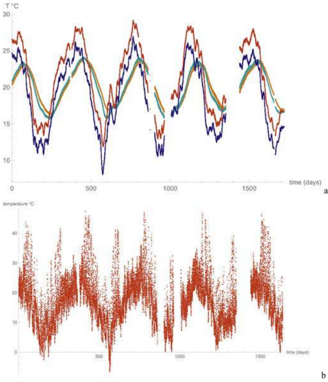
Fig. 6. - Temperature, a-in D1 (2 m: red, 6 m: orange) and D2 (2 m: dark blue, 6 m: light blue); b- in the cave (with the temperature probe) a point per hour. The series presented some gaps corresponding to some days to 2 weeks of lack of measurements. (For interpretation of the references to colour in this figure legend, the reader is referred to the web version of this article.)
