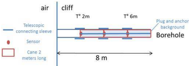
Fig. 5. - Schematic cross-section of a borehole extensometer.
