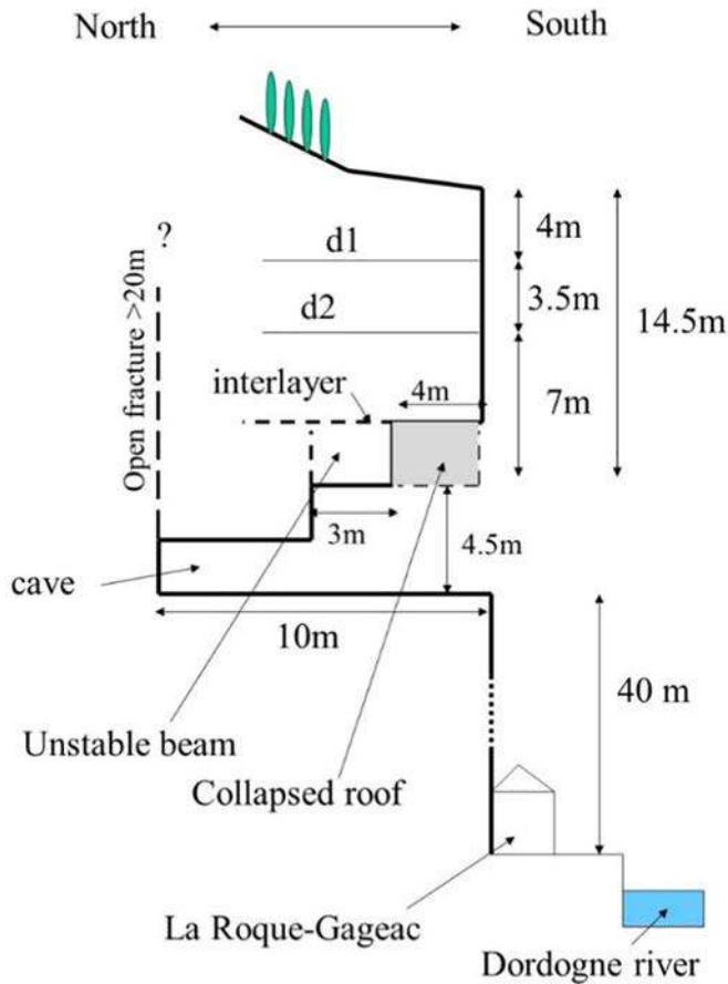
Fig. 4. – Schematic cross-section of the perched cave.
