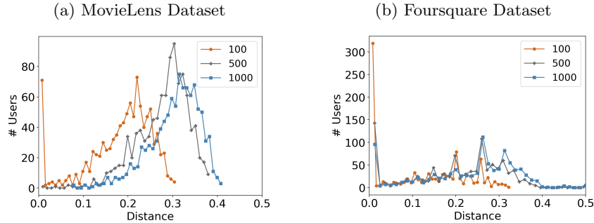
Fig. 1: Distributions of angular distances d_\theta to nearest neighbor for k = 1 for each user, plotted for vectors with dimensions 100, 500 and 1000. The distance 0.5 represents orthogonal vectors; i.e., having no items in common. The privacy guarantee for users is a function of the distance d_\theta to their nearest neighbors.
