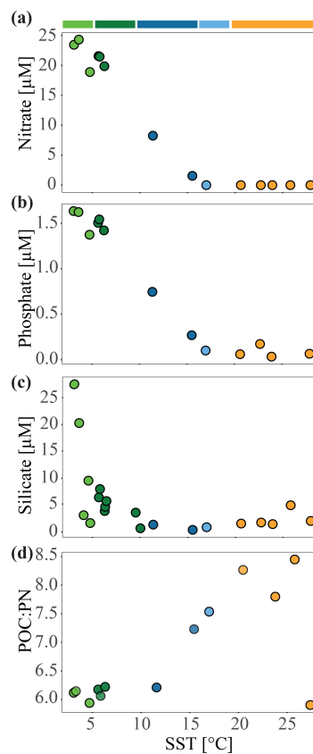
Figure 2. Nutrient concentrations ( \mu\text{mol L}^{-1} ) and molar ratios of particulate organic carbon (POC) to particulate nitrogen (PN) during the MD206 expedition against sea surface temperature (°C): (a) nitrate, (b) phosphate, (c) silicate, and (d) POC:PN ratio. Colored bars indicate water masses according to their sea surface temperature: yellow bar highlights the Indian South Subtropical Gyre (ISSG), light blue bar highlights the Subtropical Front (STF), blue bar highlights the Subantarctic Front (SAF), dark green bar highlights the Polar Front Zone (PFZ), and light green bar highlights the Antarctic Zone (AZ).
