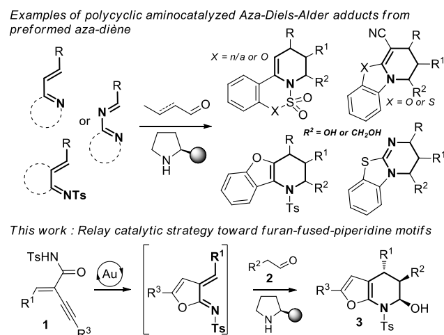
Scheme 1. Aminocatalytic HOMO-raising strategies toward polycyclic piperidines
